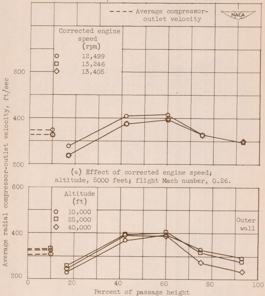
(a) Effect of corrected engine speed; altitude, 5000 feet; flight Mach number, 0.26. (b) Effect of altitude; average corrected engine speed, 13,208 rpm; flight Mach number, 0.52.
