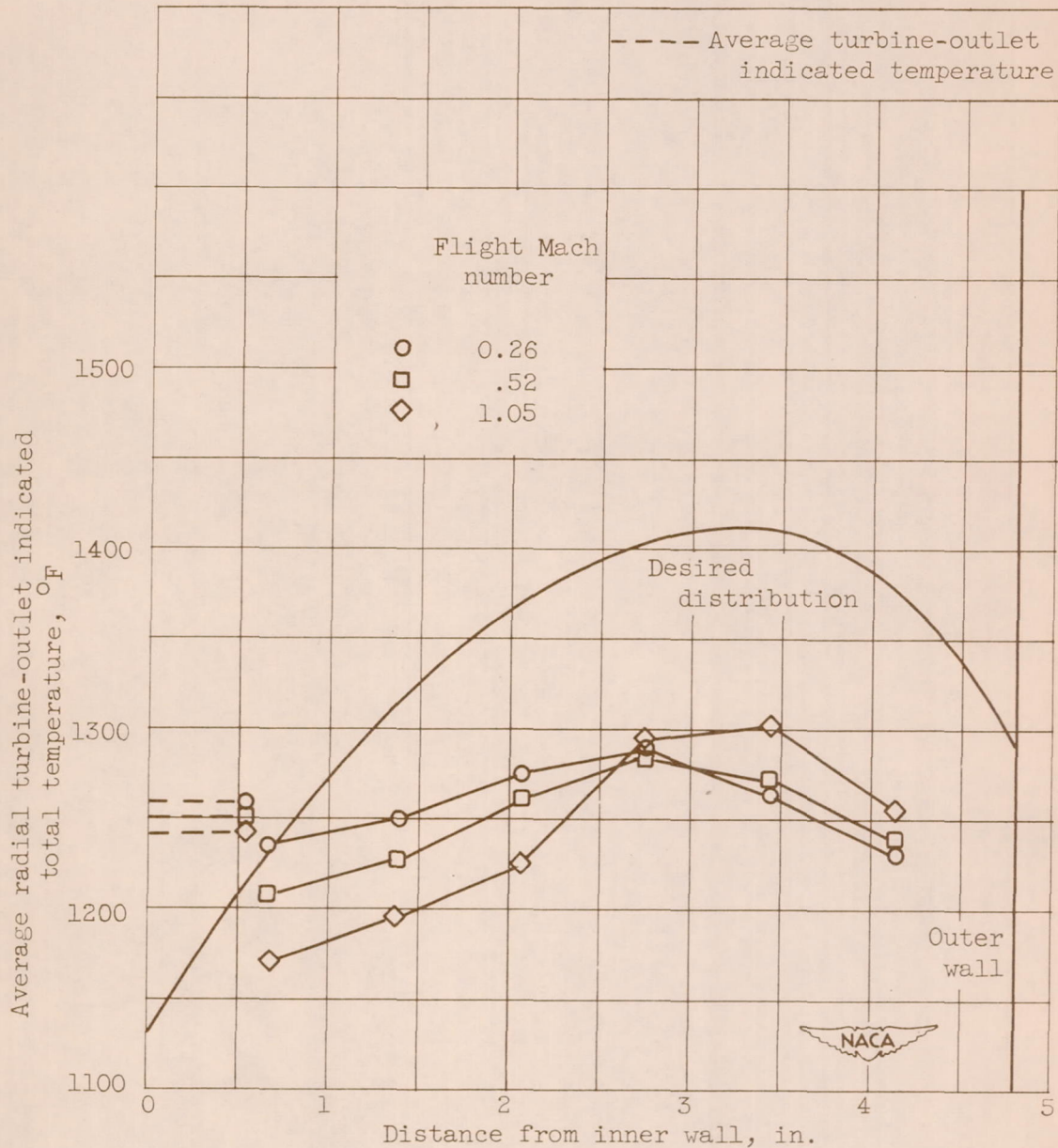
Figure 8. - Effect of flight Mach number on radial turbine-outlet temperature distribution in XJ34-WE-32 engine without mixer vanes. Altitude, 25,000 feet; corrected engine speed, 12,415 rpm.
