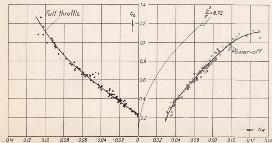
Figure 9.- Airplane polars for full throttle and power-off flight.
