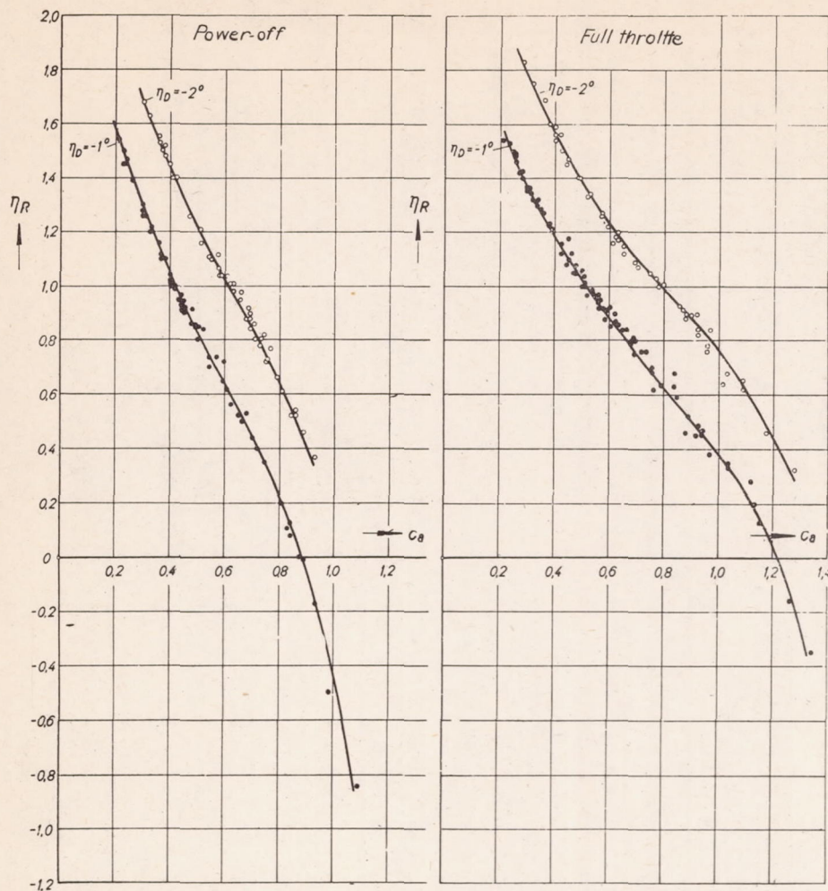
Figure 12.- Elevator angle against lift coefficient at control force moment M_{st} = 0.282 \text{ mkg} for full throttle and power-off flight.
