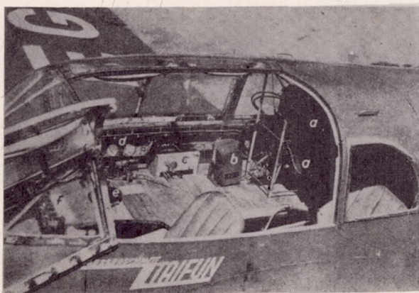
Figure 4.- View of test instruments in cockpit.
