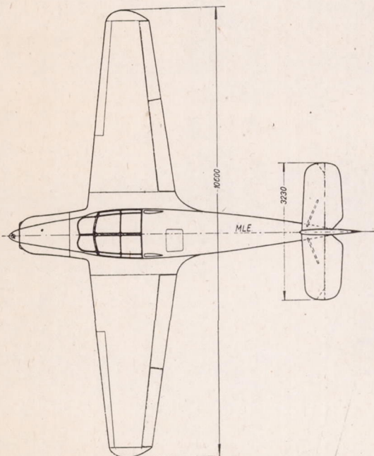
Figure 1.- Experimental airplane Bf 108.
