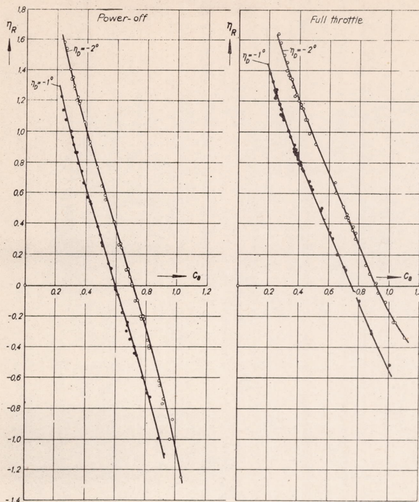
Figure 11.- Elevator angle against lift coefficient with weight-balanced elevator for full throttle and power-off flight.
