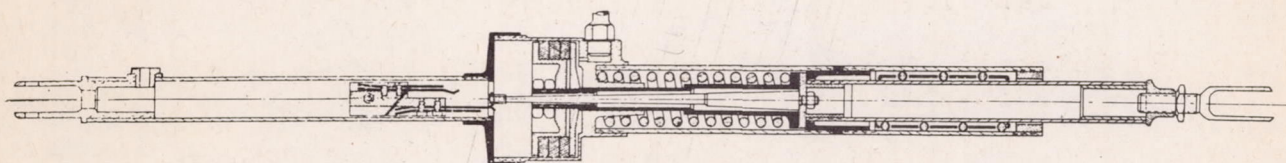
Figure 3.- Push rod uncoupling mechanism for elevator.
