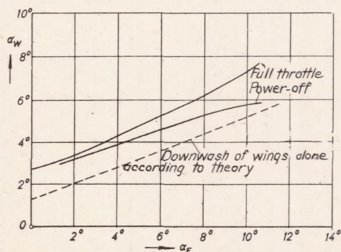
Figure 15.- Downward angle at tail as function of \alpha_F for full throttle and power-off flight.
