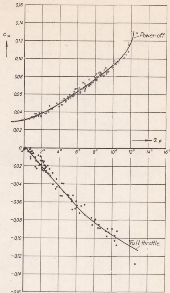
Figure 8.- Drag coefficient plotted against angle of attack of fuselage axis for full throttle and power-off flight.
