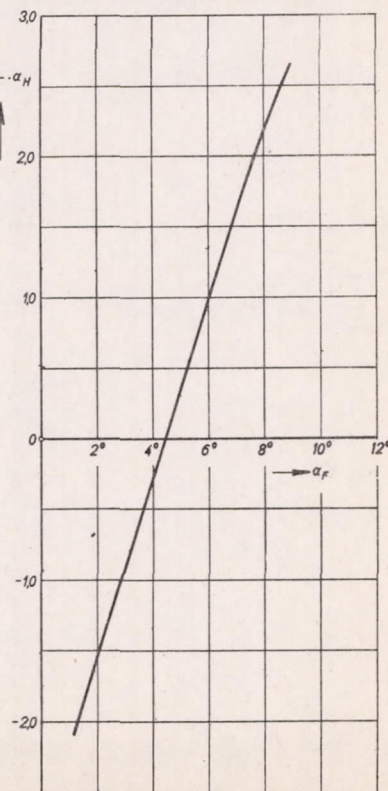
Figure 19.- Diagram for defining the tail efficiency.
