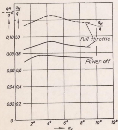
Figure 18.- Dynamic pressure at tail against angle of attack of airplane.
