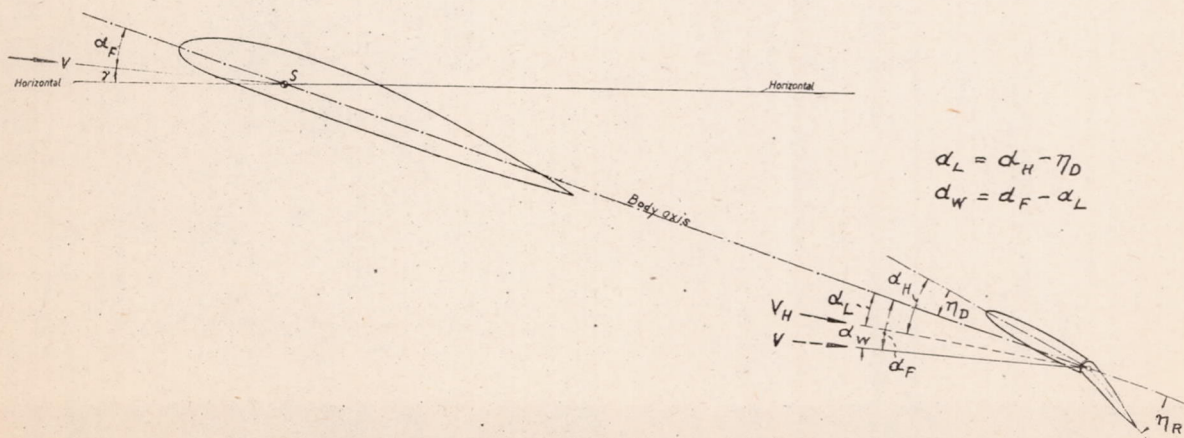
Figure 13.- Identification of angles.
