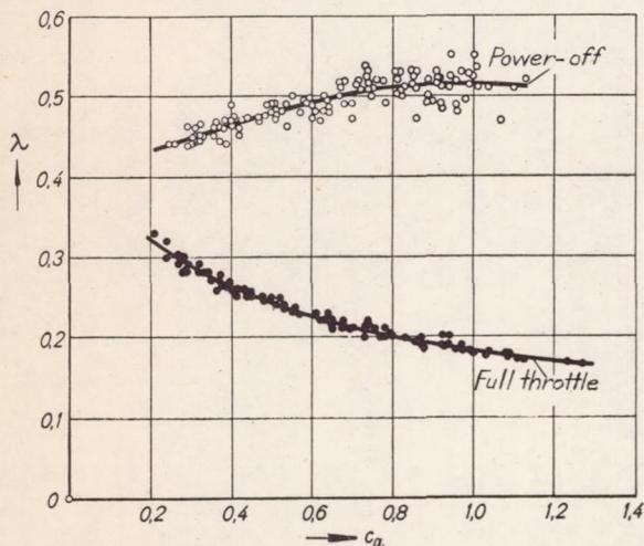
Figure 10.- Coefficient of advance against lift coefficient for full throttle and power-off flight.
