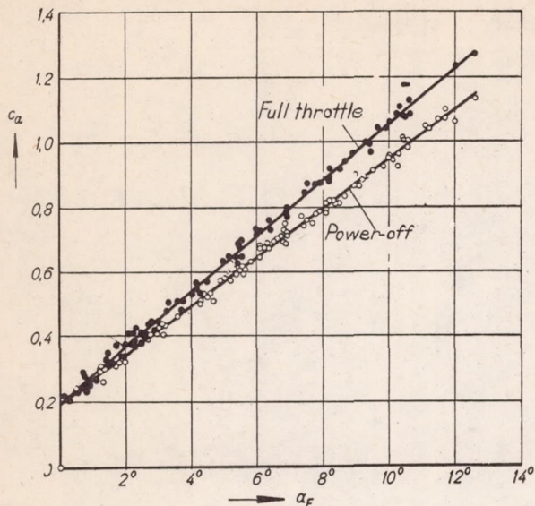
Figure 7.- Lift coefficient plotted against angle of attack of fuselage axis for power-off and full throttle flight.
