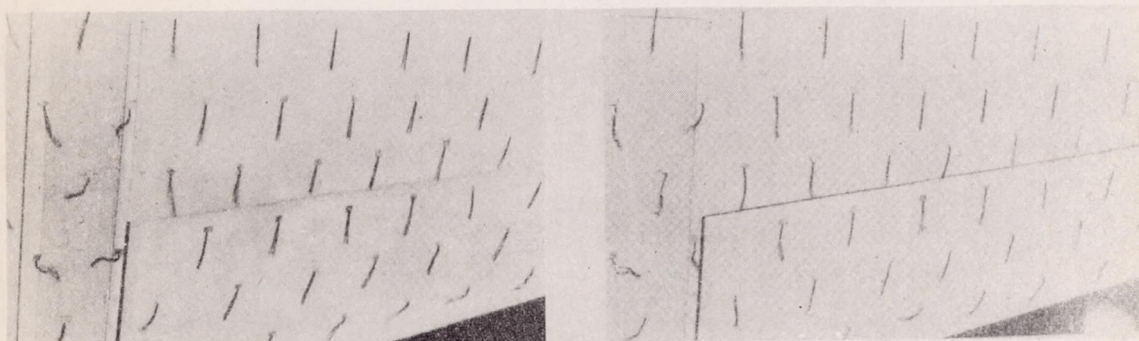
Figure 17.- Wool tuft record on inboard portion of wing at power-off flight.
