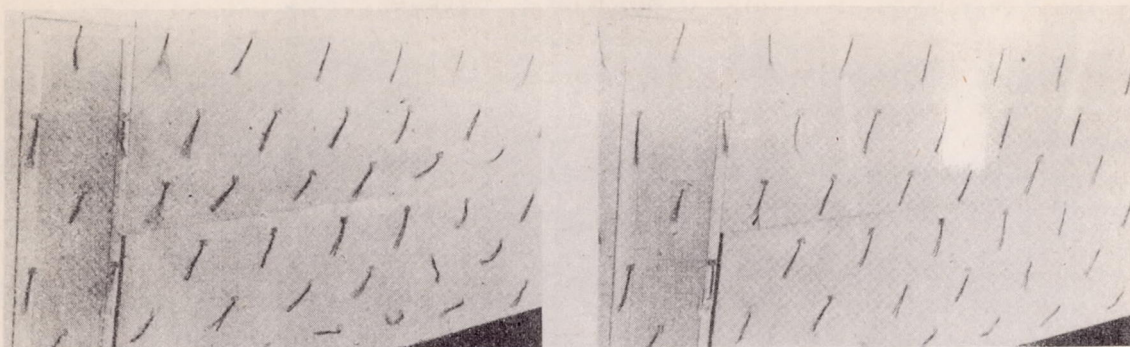
Figure 16.- Wool tuft record on inboard portion of wing at full throttle. (a) c_a = 0.925 \alpha_F = 8.4^\circ . (b) c_a = 1.275 \alpha_F = 12.3^\circ .
