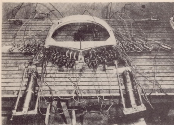
Figure 8.- Application of complementary force at the straps.
