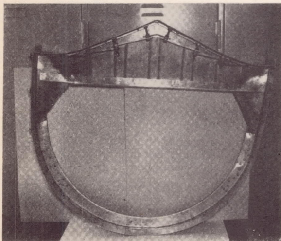
Figure 6.- Application of forces acting along frame bottom by flexibly attached straps.
