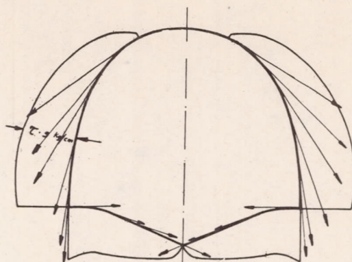
Figure 5.- Shear distri- bution over the frame and analysis in five concentrated loads.
