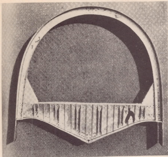
Figure 11.- View of explored frame designs.
