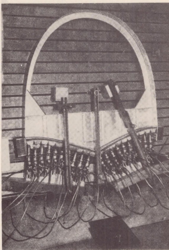
Figure 9.- Simple test rig for frames which generally give too high values and is therefore rarely used.
