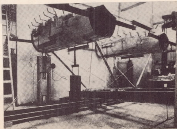
Figure 16. Arrangement for testing the strength of a flotation gear.
