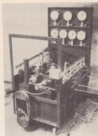
Figure 1b. Control apparatus for automatic oil pressure distribution of six oil circuits.
