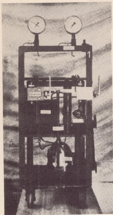
Figure 1a.- Portable oil pressure pump with controls and test instruments for two oil circuits.
