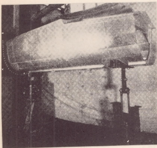
Figure 13.- Strength test of float in the case of bow impact.
