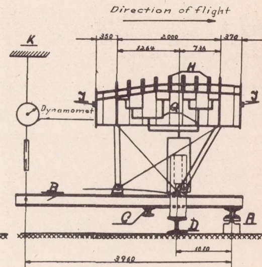
Figure 15.- Diagrammatic sketch of experimental layout for testing the strength of float supports.
