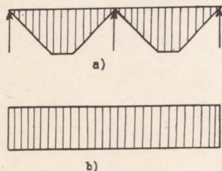
Figure 2.- (a) Mathematical bottom pressure distribution on the float frame. (b) Experimentally applied bottom pressure distribution.
