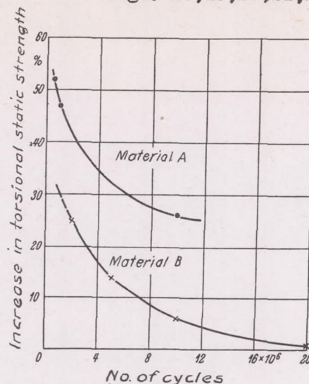
Figure 19.- Effect of pressing the hole edges on the torsional static strength of two aluminum alloy shafts with transverse holes.
