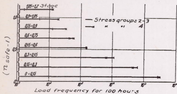
Figure 11.- Frequency of the loads in multiples of (n_{safe}-1) for 100 operating hours (computed for a flight velocity of 350 km/h); (n_{safe}-1) is the safe load which due to gusts is added, according to the structural requirements, to the load in the undisturbed and unaccelerated rectilinear flight for airplanes.
