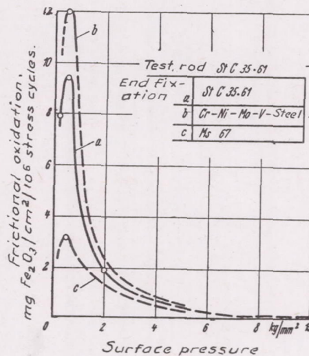
Figure 21.- Frictional oxidation as a function of surface pressure and material saving in the juncture for St C 35.61.
