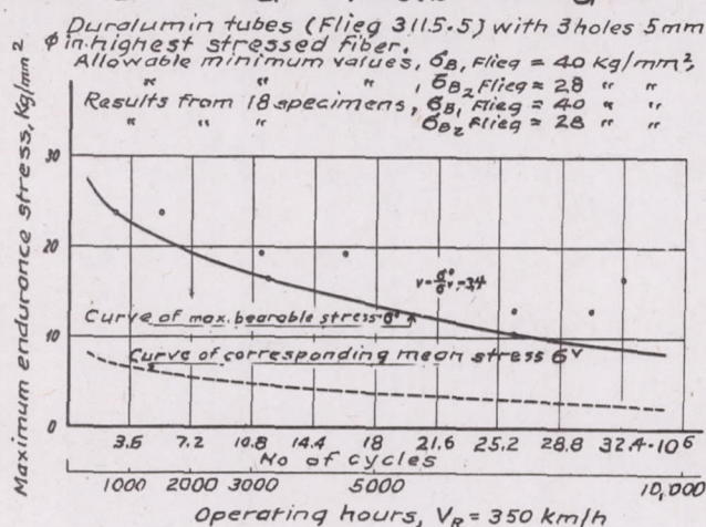
Figure 16.- Stress curve for duralumin tubes with 3 holes (5 mm diam) in the maximum stressed fibers (E. Gassner).
