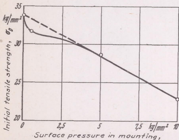
Figure 22.- Tensional strength as a function of the surface pressure in the juncture for St C 35.61.
