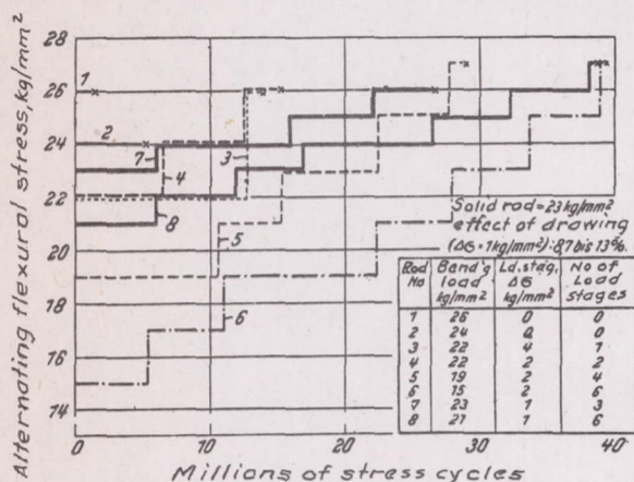
Figure 14.- Variation of the flexural fatigue strength through understress effect, unalloyed steel with 0.2 percent C (F. Körber).
