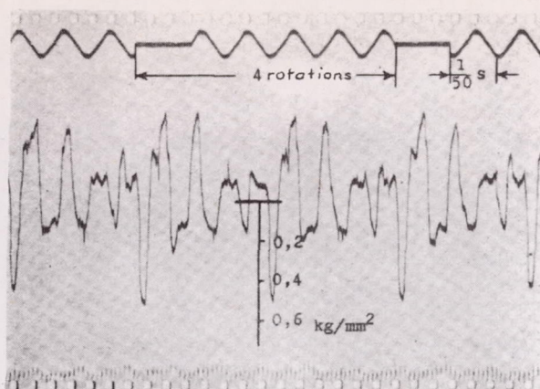
Figure 8.- Record of stress at a propeller blade root, measured with the instrument shown in fig. 7. (BMW 132 engine, n=2150 rpm).
