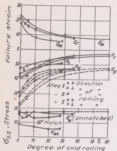
Figure 18.- Dependence of strength properties on the degree of cold rolling for several aluminum alloys.
