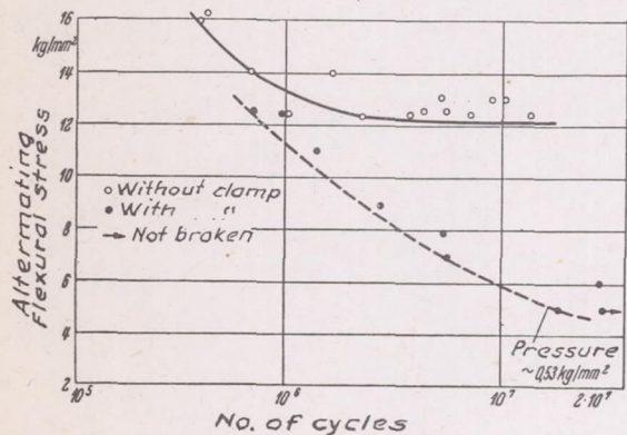
Figure 20.- Effect of end fixation on the Wöhler strength of an aluminum alloy (Al-Cu-Mg) for alternating bending stress (W. Müller).
