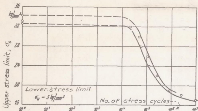
Figure 1.- Wöhler curve for an aluminum alloy with 6 percent Mg and 1 percent Zn.
