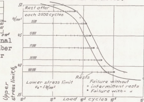
Figure 5.- Effect of intermittent rests on the Wöhler strength of an austenitic chrome-nickel steel (18 percent Cr, 8 percent Ni).
