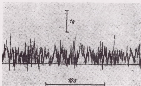
Figure 10.- Acceleration due to vertical gusts of an airplane in cruising (He 70, UDAS).
