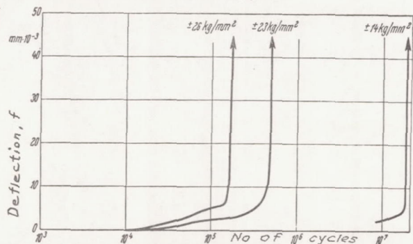
Figure 4.- Dependence of the flexural strain on the number of load cycles for duralumin.
