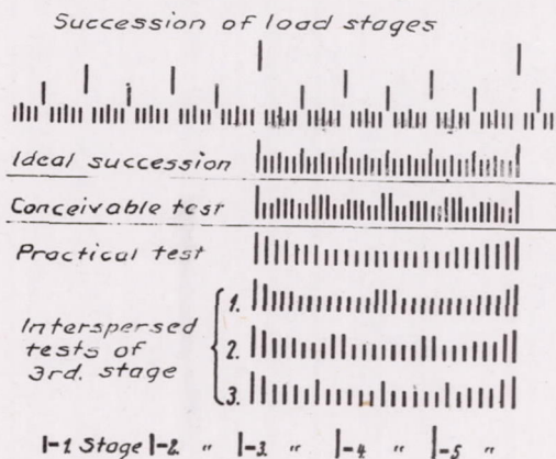
Figure 12.- Sequences of load stages (A. Teichmann).
