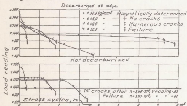
Figure 3.- Dependence of the torsional stress limits on the number of load cycles for tension wires for various strain limits.
