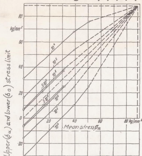
Figure 2.- Limited time and fatigue strength diagram for heat treated chrome-molybdenum steel tubes, aviation material 1452, with a transverse hole of 2 mm diameter.
