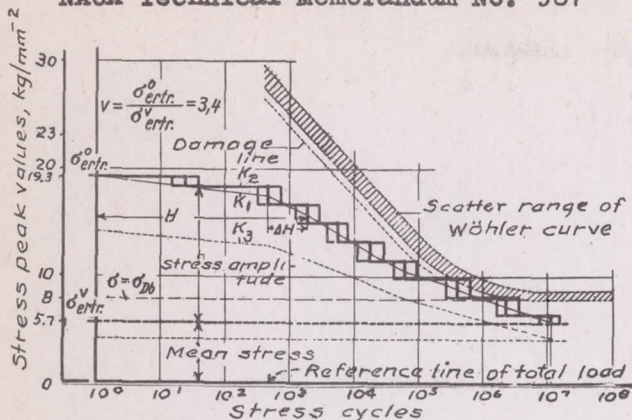
Figure 13.- Results of a statistical strength test (E. Gassner). Test specimen: Duralumin tube 50.1 (aviation material 3115) with 5 mm hole in the maximum stressed fibers; \sigma_B = 46 \text{ kg/mm}^2 , \sigma_{0.2} = 34 \text{ kg/mm}^2 (admissible minimum values for material \sigma_B = 40 \text{ kg/mm}^2 , \sigma_{0.2} = 28 \text{ kg/mm}^2 )
