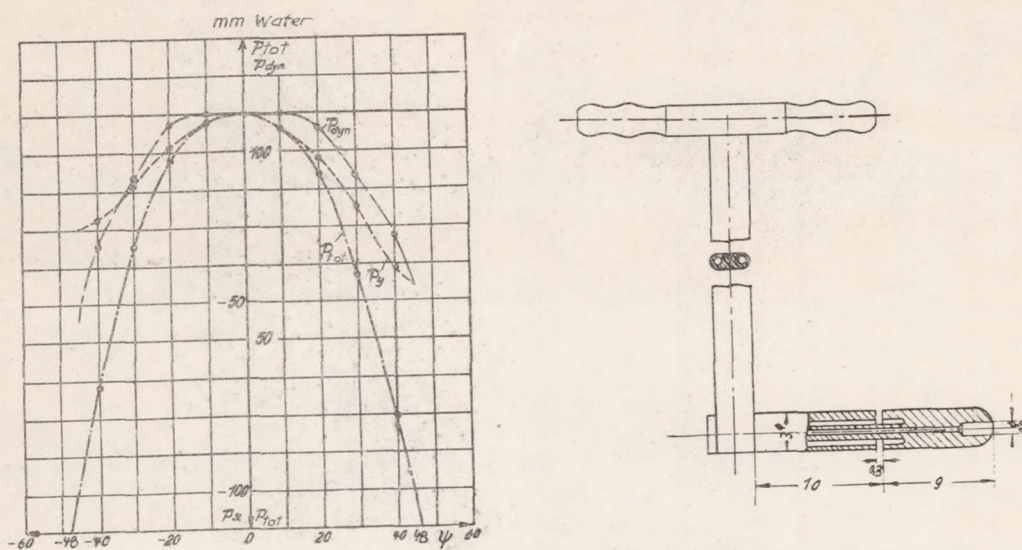
Figure 2.- Prandtl pitot and pressure variation obtained by yawing the total head tube.
