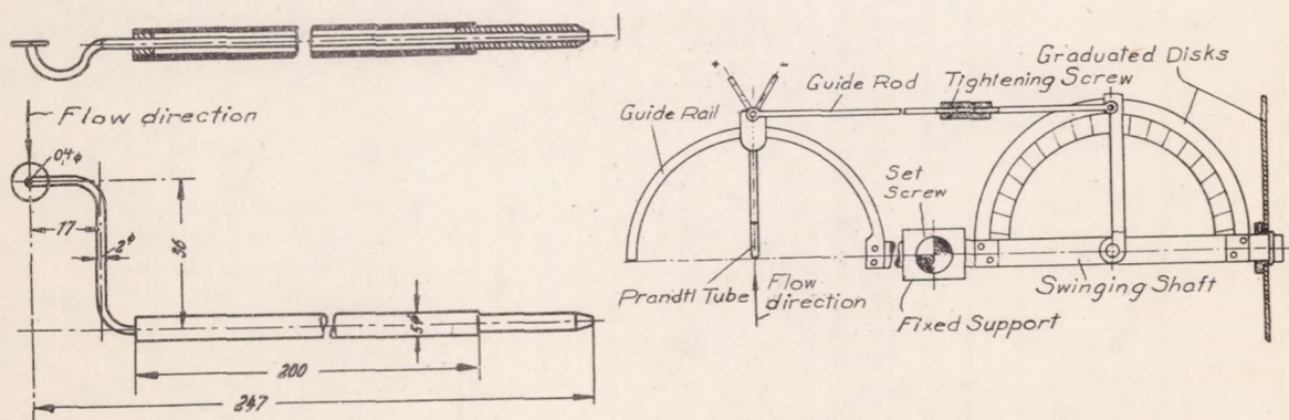
Figure 2.- Prandtl pitot and pressure variation obtained by yawing the total head tube.
