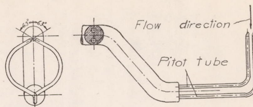
Figure 6.- Flow direction instrument consisting of two pitot tubes set at 63°.
