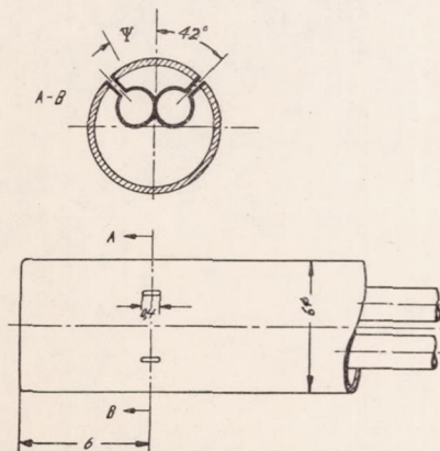
Figure 7.- Cylindrical tube used for recording two-dimensional flows and pressure variation on the cylinder surface in relation to angle of yaw.
