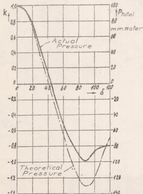
Figure 12.-Calculated and actual pressure curves.
