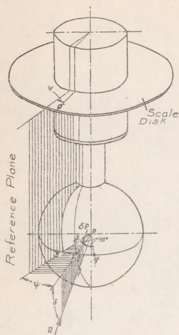
Figure 10.-Principle of spherical pitot, (identification of angles).
