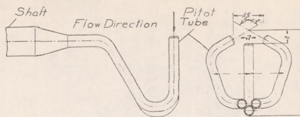
Figure 8.-Pressure recorder with 3 pitot tubes.
