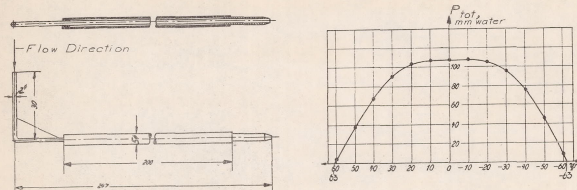
Figure 1.- Pitot tube and pressure variation for the impact opening by yawing.
