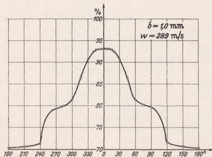
Figure 45.-Design 1; effect of flow direction.
