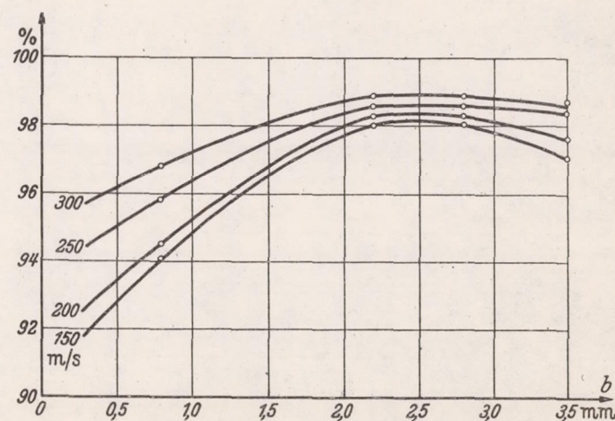
Figure 41.- Results obtained with k (Fe--Ko).
