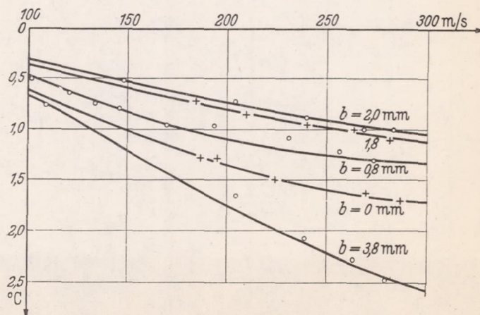
Figure 23.-Results obtained with f.
