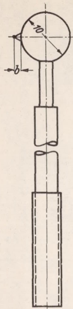
Figure 42.- Design 1.
