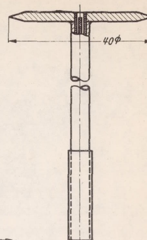
Figure 51.- Plate thermometer.
