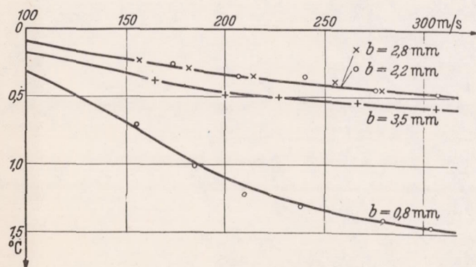
Figure 40.- Results obtained with k (Fe--Ko).
