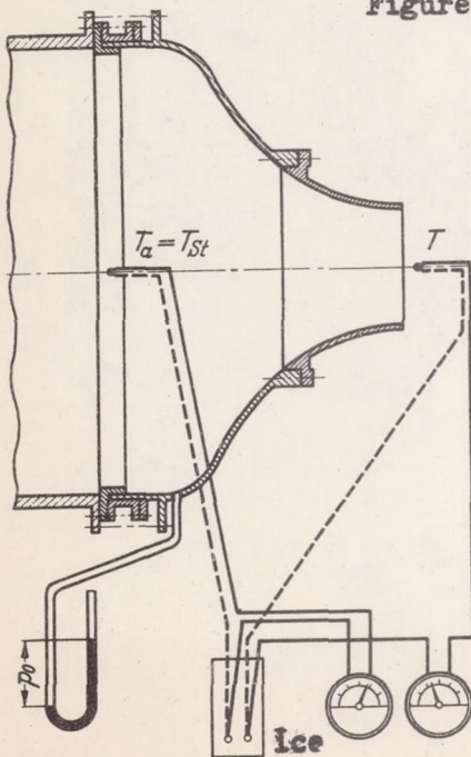
Figure 4.-Test stations.
