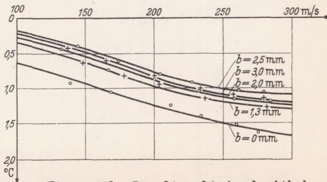
Figure 31.- Results obtained with h.
