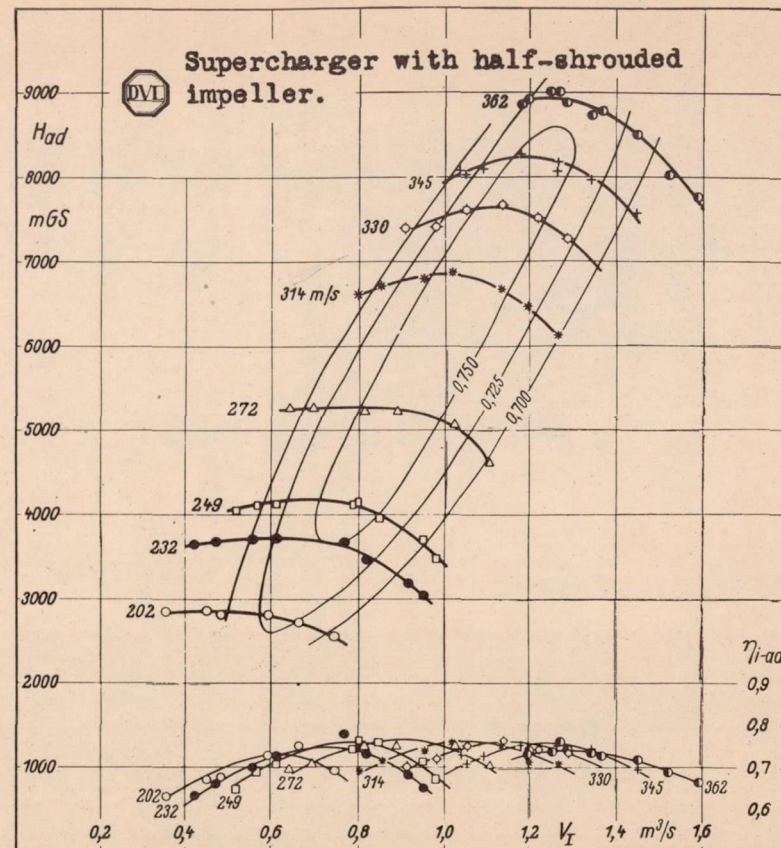
Figure 3.- Characteristics of a DVL supercharger.
