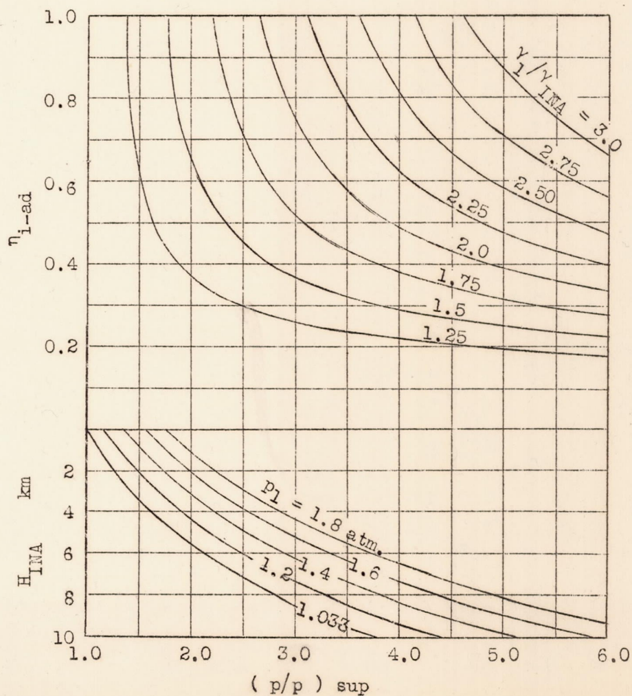
Figure 12.- Effect of supercharger efficiency on the increase in density.
