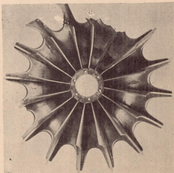
Figure 8.- Impeller failures with impeller wall cut-outs.
