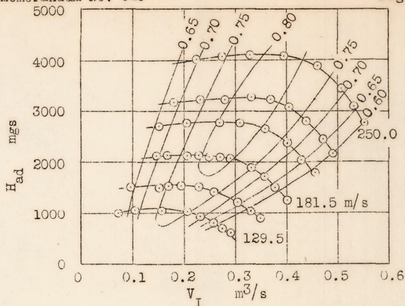
Figure 6.- Characteristics of a small DVL supercharger.
