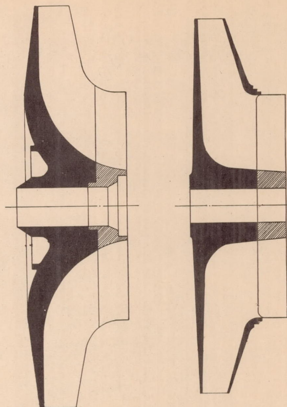
Figure 7.- Impellers: left, Rolls-Royce(3 kg), right, DVL (1.3 kg).
