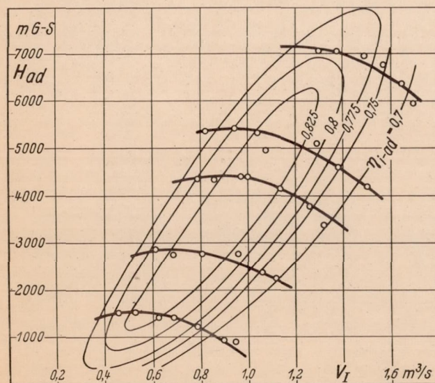
Figures 1 and 2.- Characteristics of various DVL superchargers.
