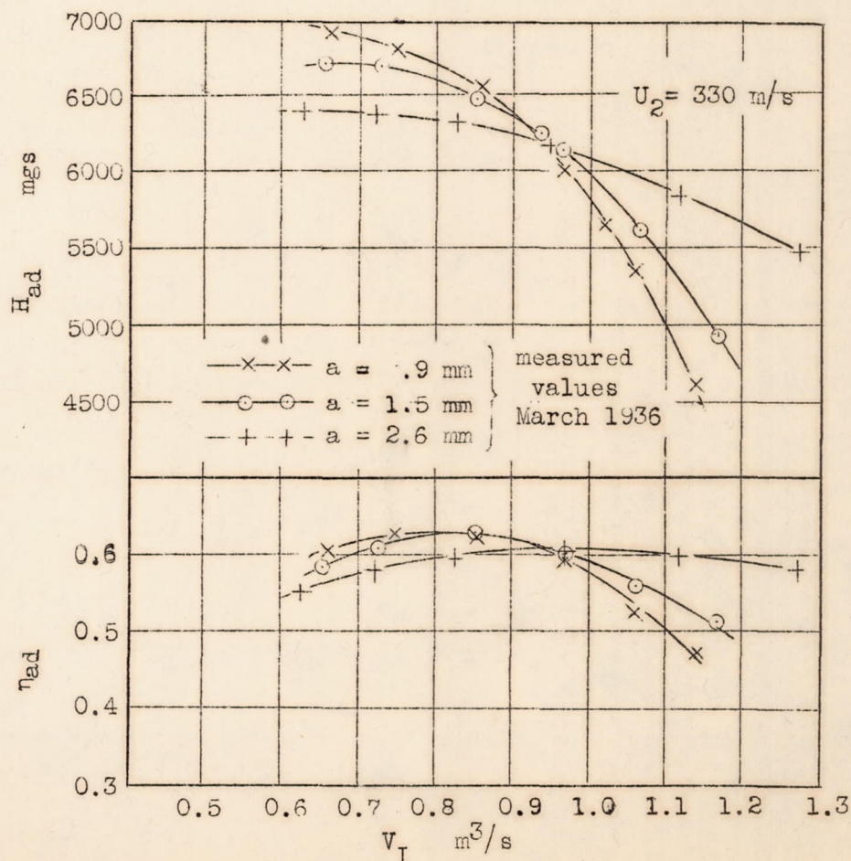
Figure 9.- Effect of cover clearance.
