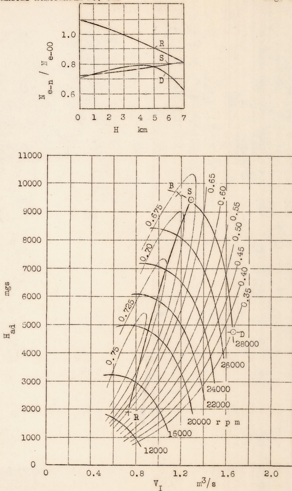
Figure 10.- Engine operating points in the region of supercharger characteristics and engine powers ( in graph above ).
