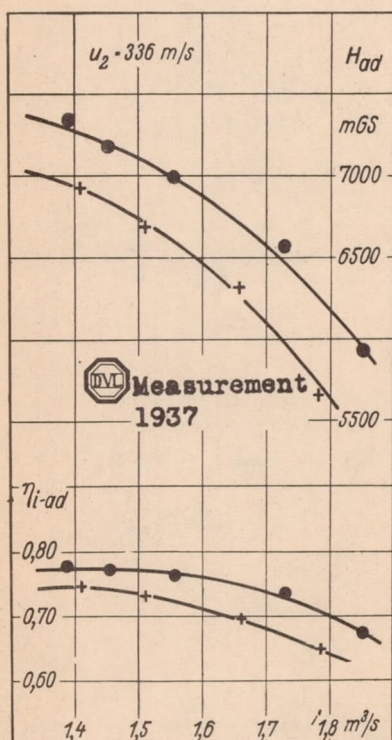
Figures 4 and 5.- Comparison of half-shrouded with shrouded impeller.
