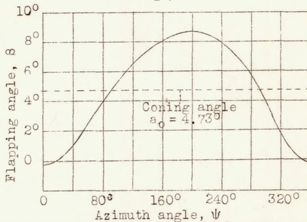
Figure 9.- Flapping angle as a function of the azimuth angle for G = 900 kg and \mu = 0.4 .
