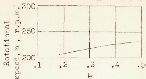
Figure 7.- Rotational speed as a function of \mu for G = 900 kg.
