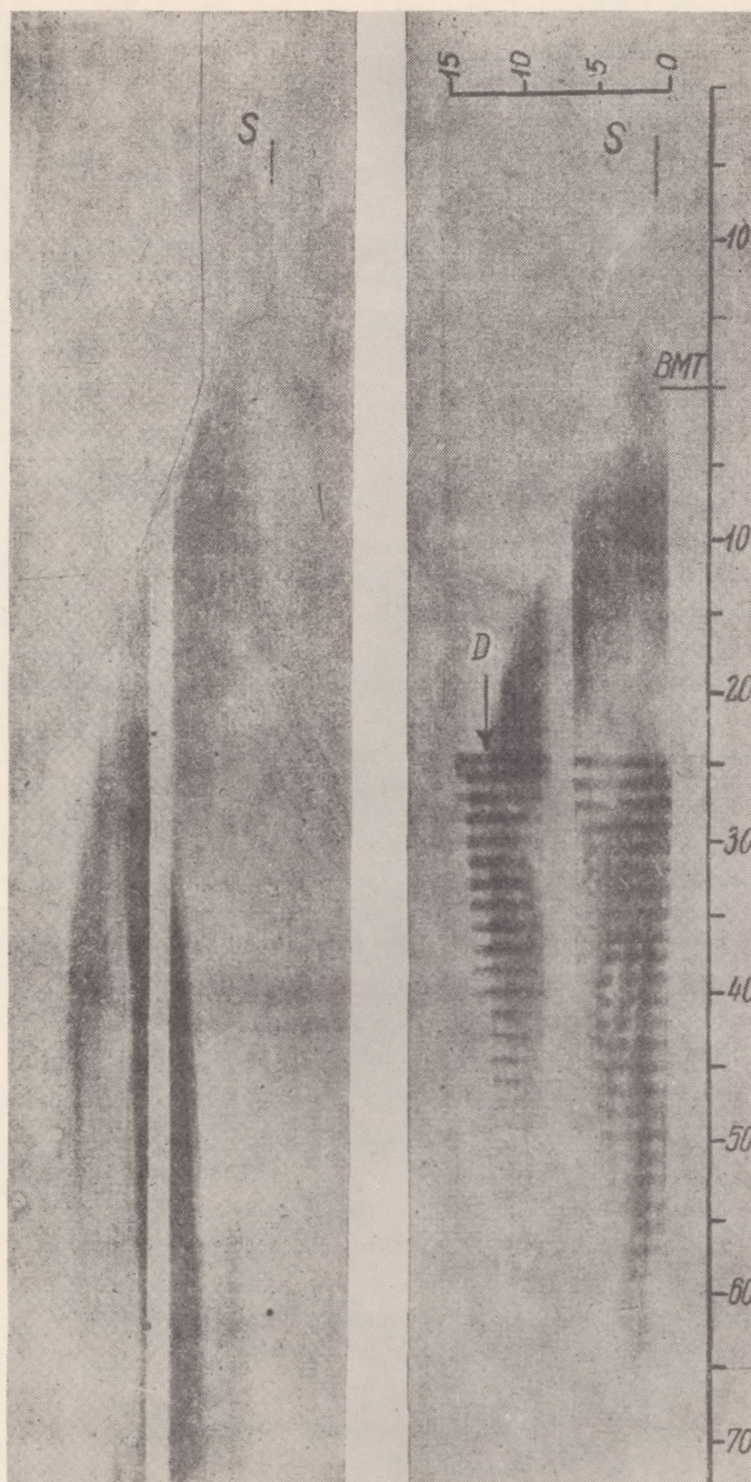
Figure 3.- Photo-records of normal combustion (A) and with detonation (B) in the engine. C- spark. D- point at which detonation is initiated.
