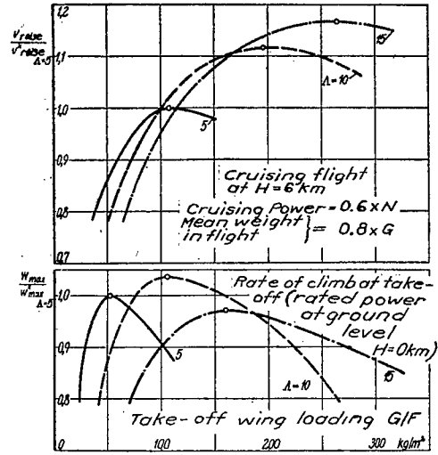
Figure 22.- Long range airplane (with weight correction; G'F'/G' = 0.14 ). G = 32000 kg; N = 4 \times 1000 hp,
