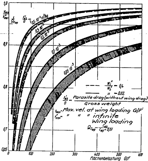
Figure 20.- Dependence of the maximum speed on the wing loading at equal span loading v_{max0} = 400 km/h; ( v_{cruis} * \Lambda = 5 = 295 km/h) G/b^2 (without weight correction).
