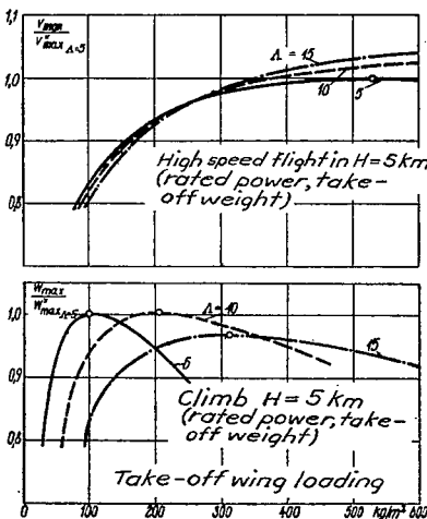
Figure 21.- Design magnitudes of airplanes of the years 1935 to 1937.
