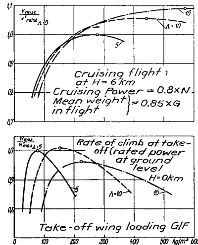
Figure 23.- Medium range airplane (with weight correction; G'F'/G' = 0.14 ) G = 9000 kg; N = 2 \times 1000 hp, v_{max0} = 500 km/h ( v_{cruis} * \Lambda = 5 = 480 km/h).
