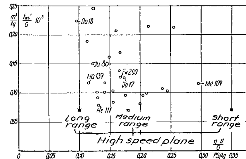
Figure 21.- Design magnitudes of airplanes of the years 1935 to 1937.
