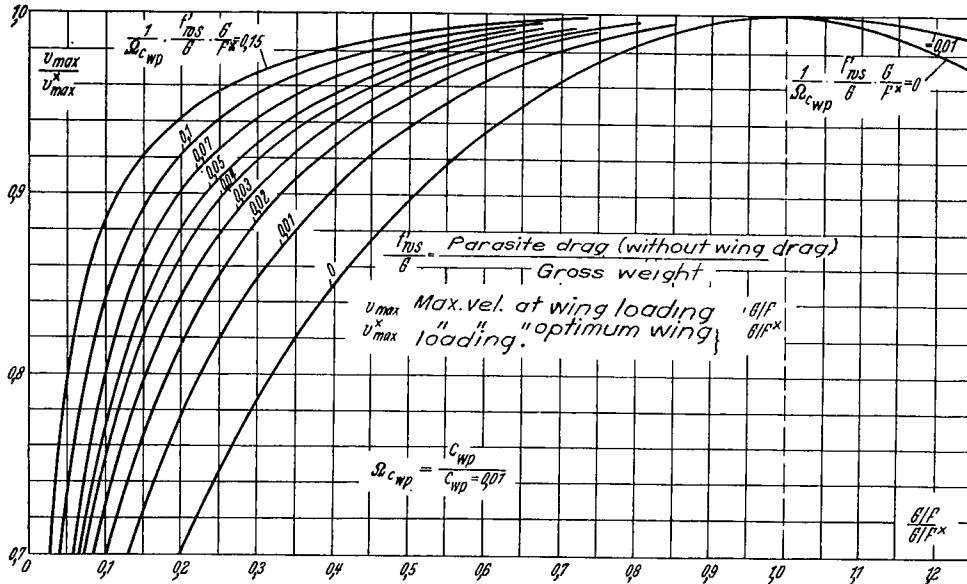
Figure 8.- Dependence of the maximum speed on the wing loading for equal aspect ratio (without weight correction).
