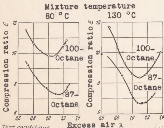
Test conditions correspond to CFR eng. method. Knock characteristics 50
