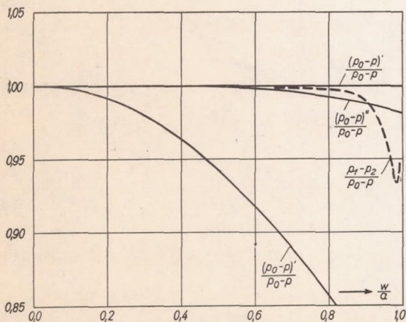
Fig. 8.- Approximate solutions of pressure gradient necessary to adiabatic formation of flow from rest position (eq. 8a, 8b) compared to pressure record p_1 - p_2 with Prandtl pitot tube.
