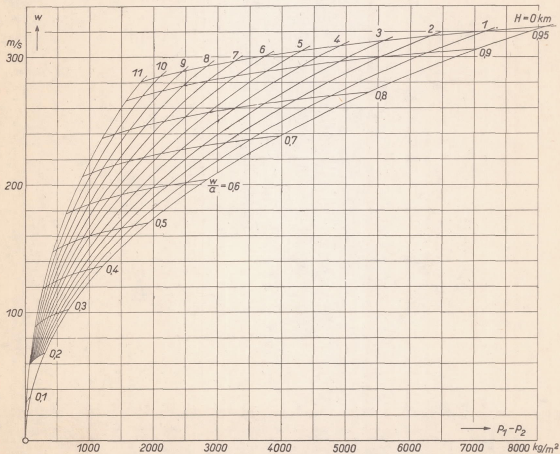
Figure 9.- Correlation of eq. (9) for flight at standard altitude.
