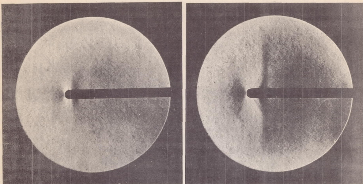
Figure 3.- Schlieren record at w/a = 0.85 .
