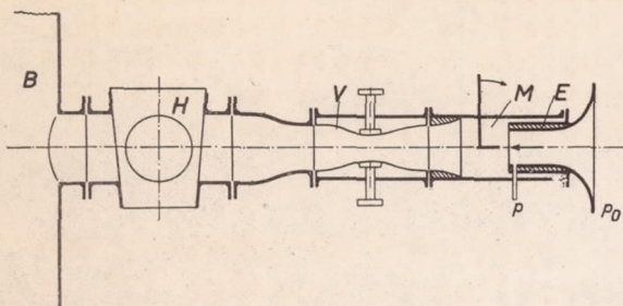
Fig. 1.- Prandtl type high-speed wind tunnel.
