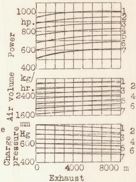
Figure 8.- Change of charge pressure against exhaust back pressure.
