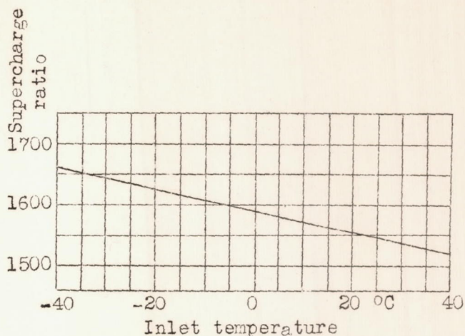
Figure 16.- Change of supercharge ratio at rated altitude plotted against inlet temperature.
