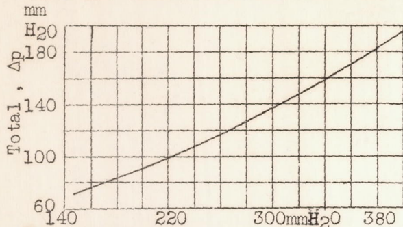
Figure 5.- Relation between pressure jump corresponding to the usual speed measured in the altitude test chamber and the total pressure jump between entry and exit from the cowl.
