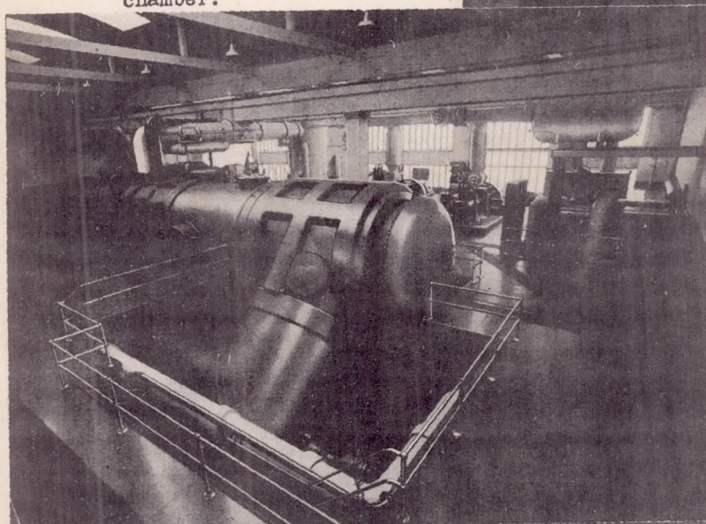
Figure 1.- Views of Fiat altitude test chamber.
