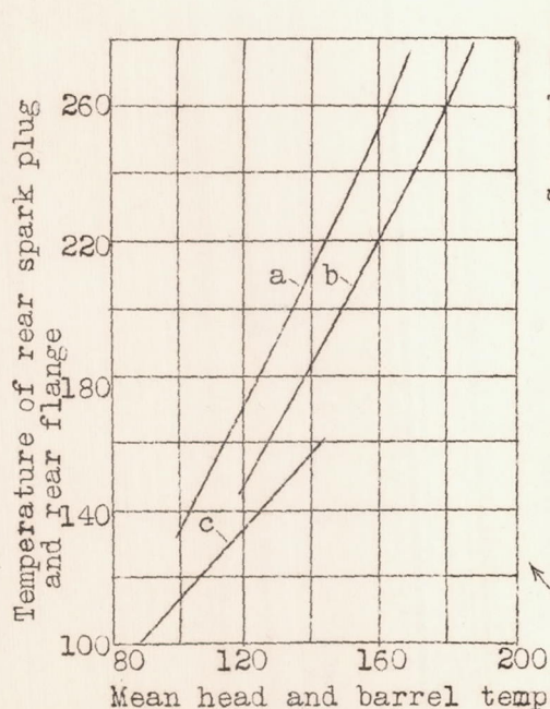
Figure 19.- Relation between the temperature of the rear spark plug and the cylinder flange on one side and the mean temperature of cylinder head, flange and total cylinder.
