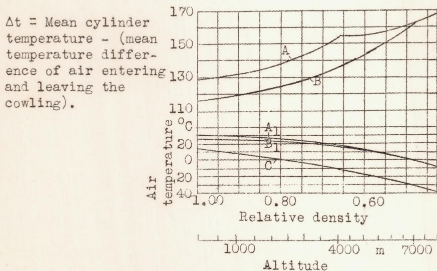
Figure 23.- Temperature variation in rear spark plug in climb in standard air at constant charge pressure.
