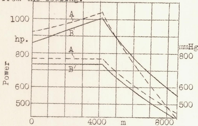
Figure 7.- Change of hp. and feed pressure at full throttle against altitude. Vacuum tank measurements versus altitude test chamber.
