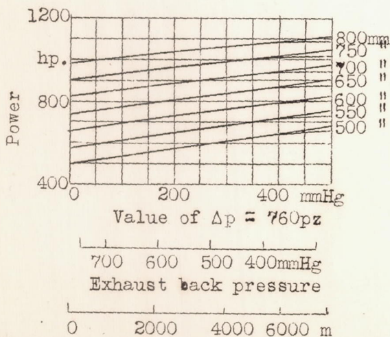
Figure 10.- Variation of power against exhaust back pressure.
