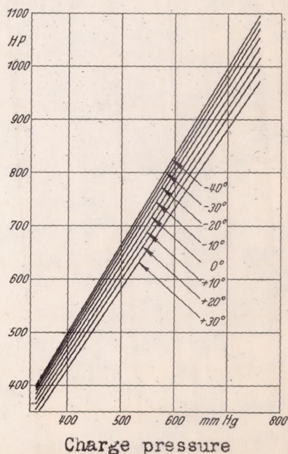
Figure 12.- Calibration curves of rated altitude at inlet temperatures ranging from -40 to +30^{\circ}
