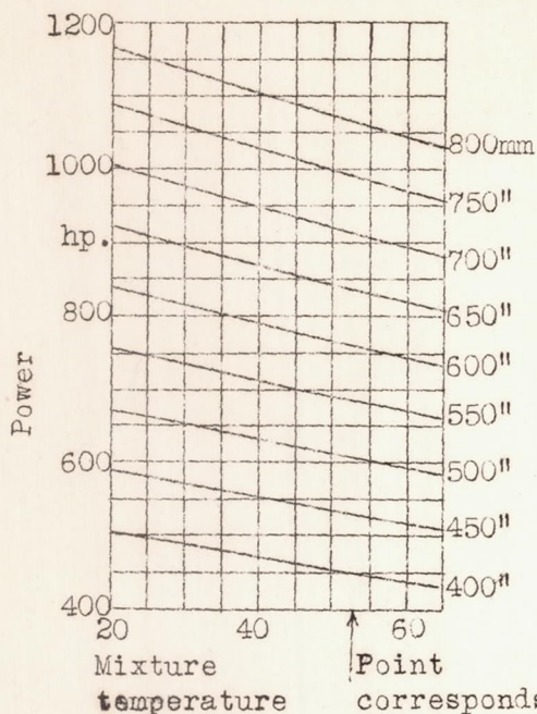
Figure 13.- Variation of power plotted against mixture temperature.
