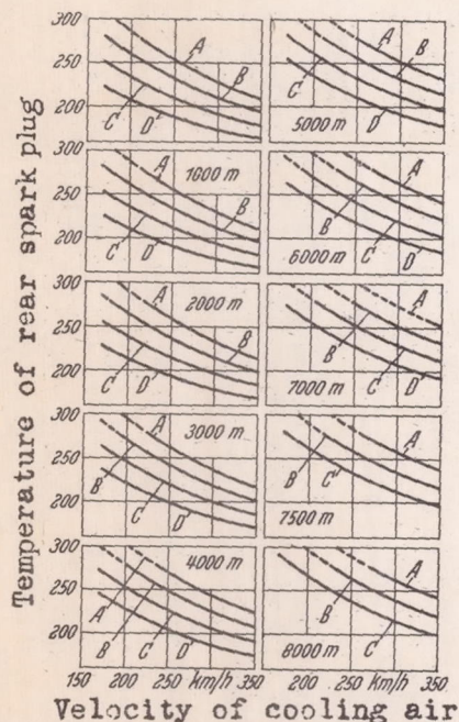
Figure 20.- Temperature variations of the rear spark plug at constant output at different heights and different wind velocities.
