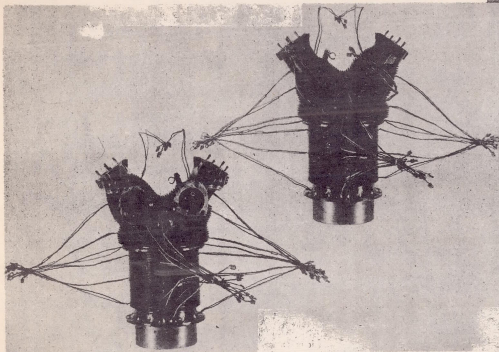
Figure 18.- Distribution of thermocouples for recording the mean cylinder temperature.
