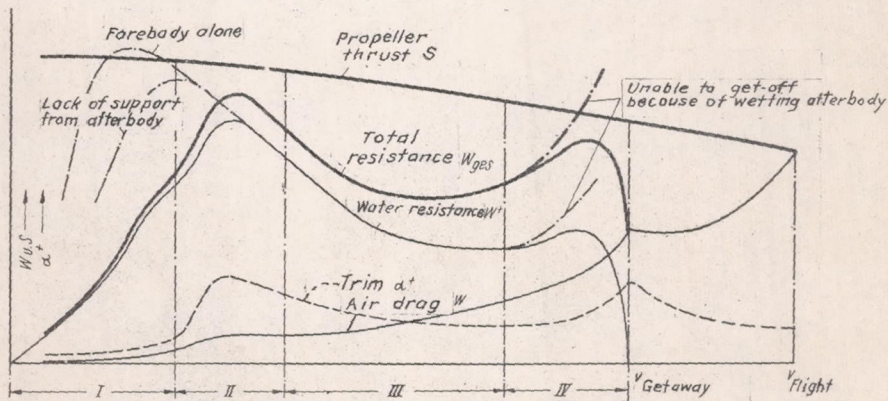
Figure 3.- Take-off diagram.
