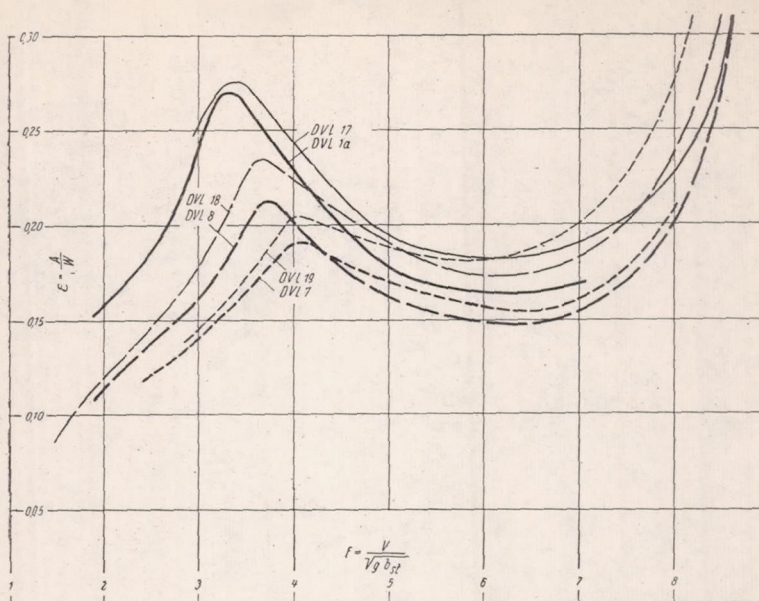
Figure 20.- Optimum resistance for all models at the same load.
