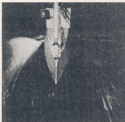
Figure 12.- Deflection of spray; left half: form of section according to figure 11c, right " " " " " " " 11b.
