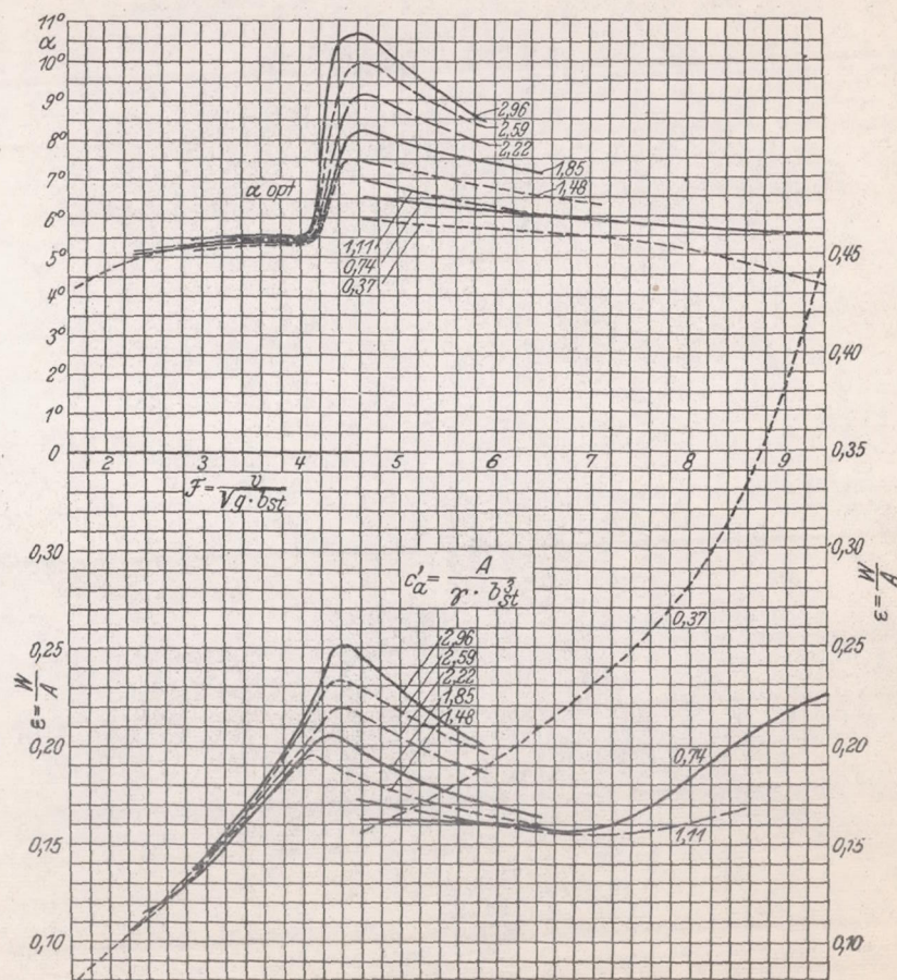
Figure 17.- Optimum resistance and the corresponding trim (best trim).
