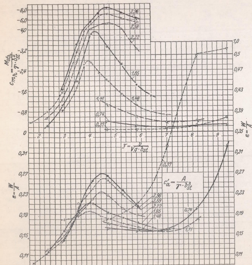
Figure 16.- Resistance and moments; example for DVL 7, \alpha = 7^\circ const.
