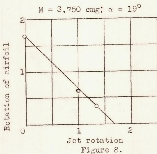
Figures 7, 8.- Jet rotation substituted for airfoil rotation.
