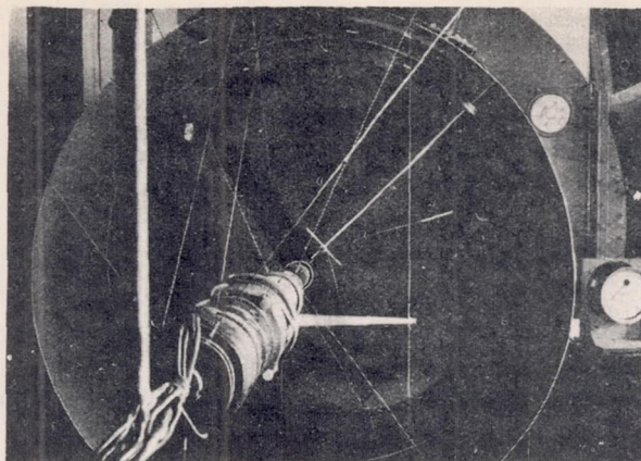
Figure 4.- Model airfoil mounted on rotation device.
