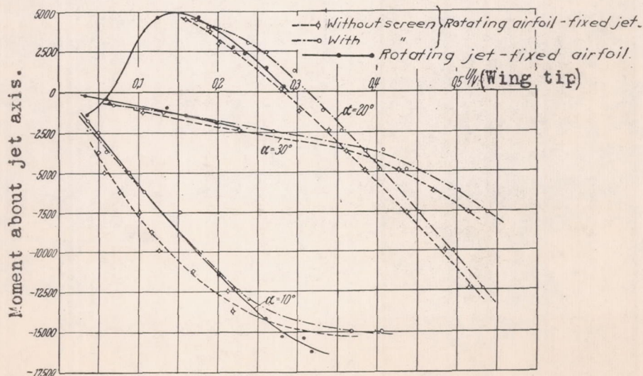
Figure 11.- Spinning moments of airfoil section M5.
