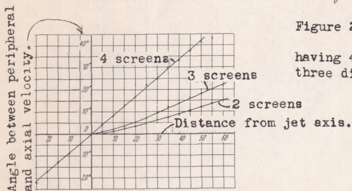
Figure 3.- Radial tip speed distribution for different screen speeds.
