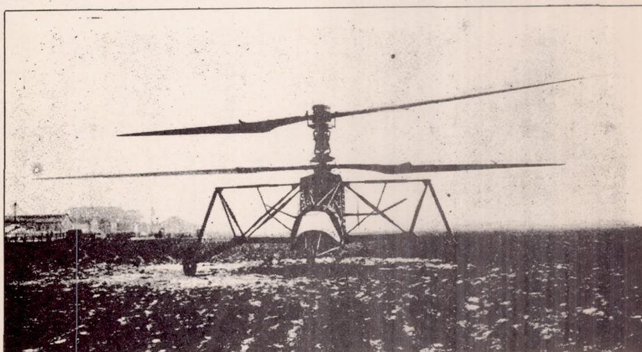
Figure 6.- 1935 experimental gyroplane.
