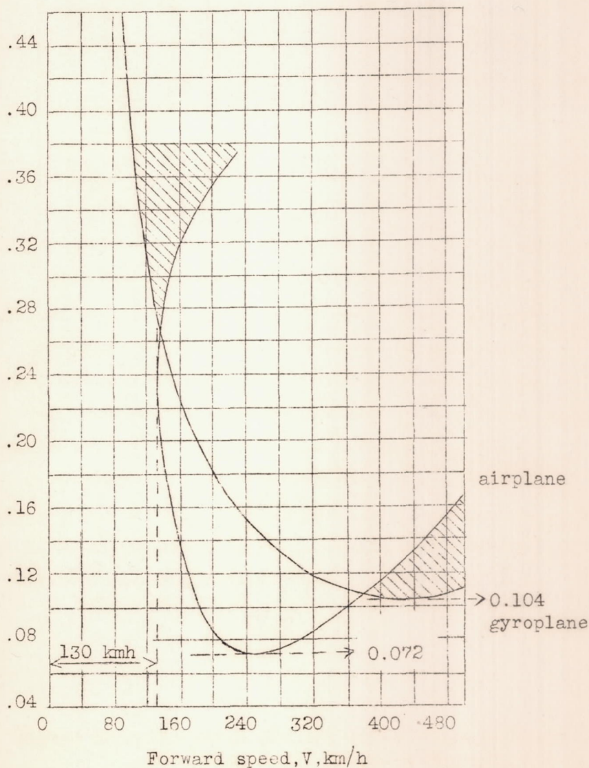
Figure 15.- Gyroplane of the future ( \sigma/P^2 = 1/15000 ) and airplane of exceptional aerodynamic qualities.
