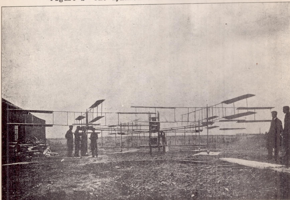
Figure 4 The gyroplane of 1907
