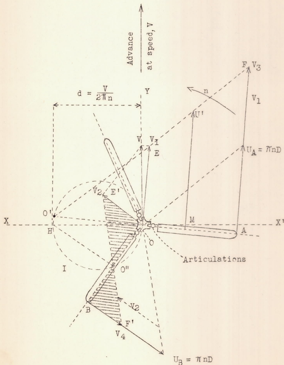
Figure 7.- Distribution of speed and reversed-velocity region for a propeller revolving at rate n and advancing at speed V .
