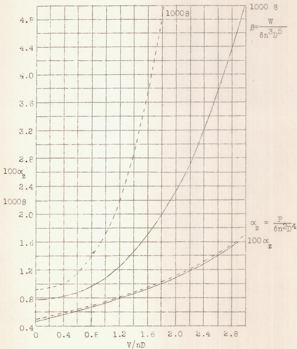
Figure 11.- Gyroplane. Lift and power coefficients.
