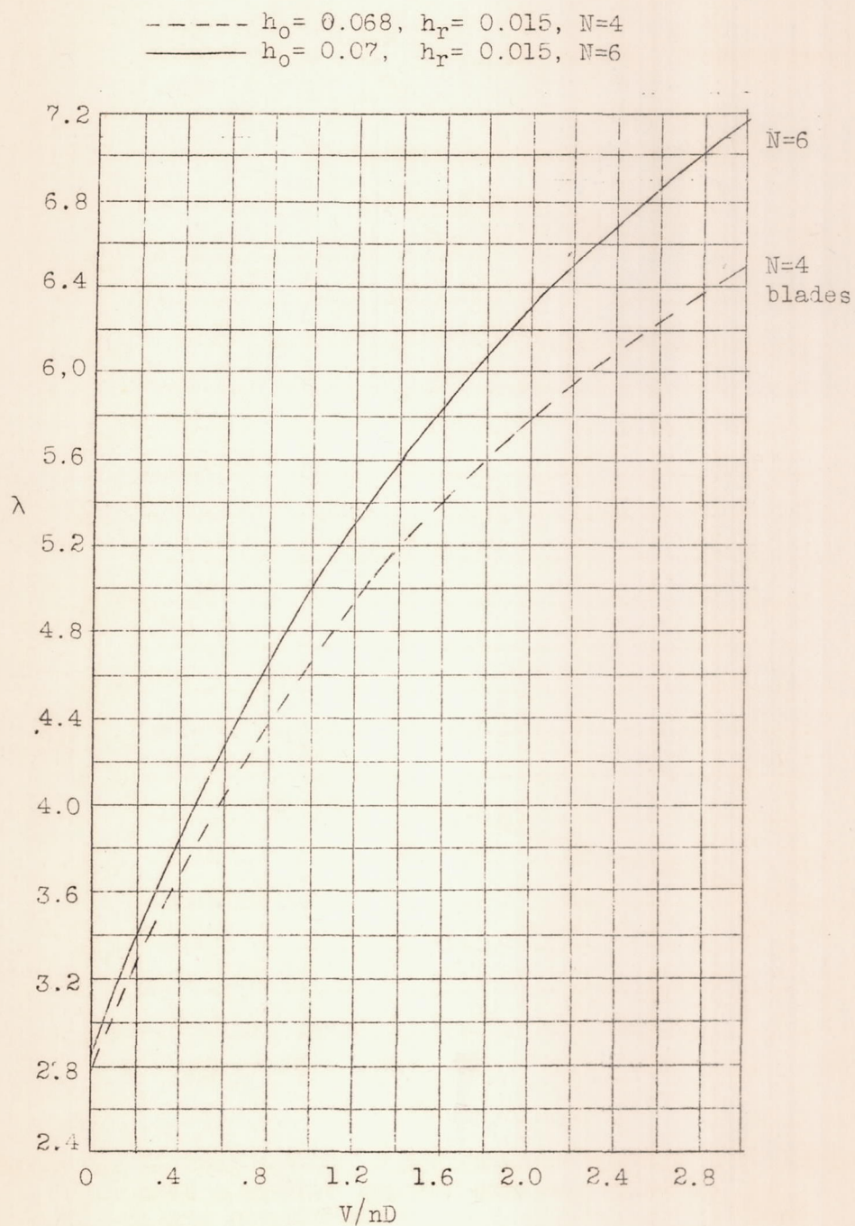
Figure 9.- Gyroplane.- Effective aspect ratio \lambda of a blade.
