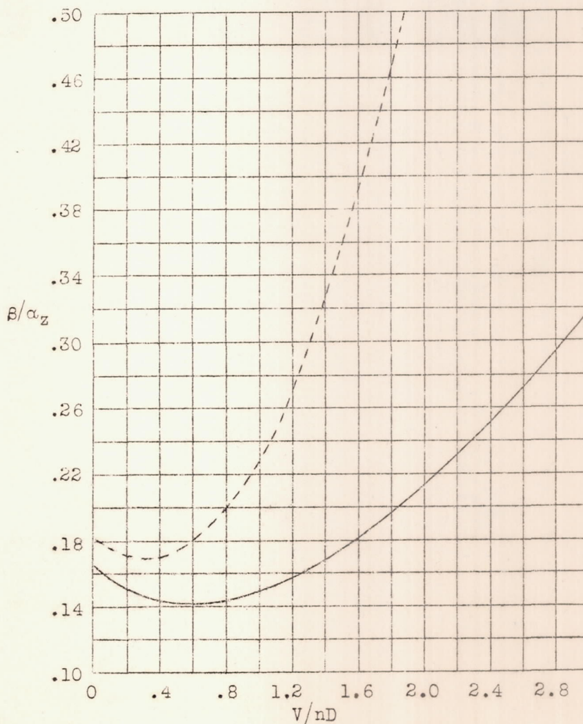
Figure 18.- Coefficient of propeller torque.
