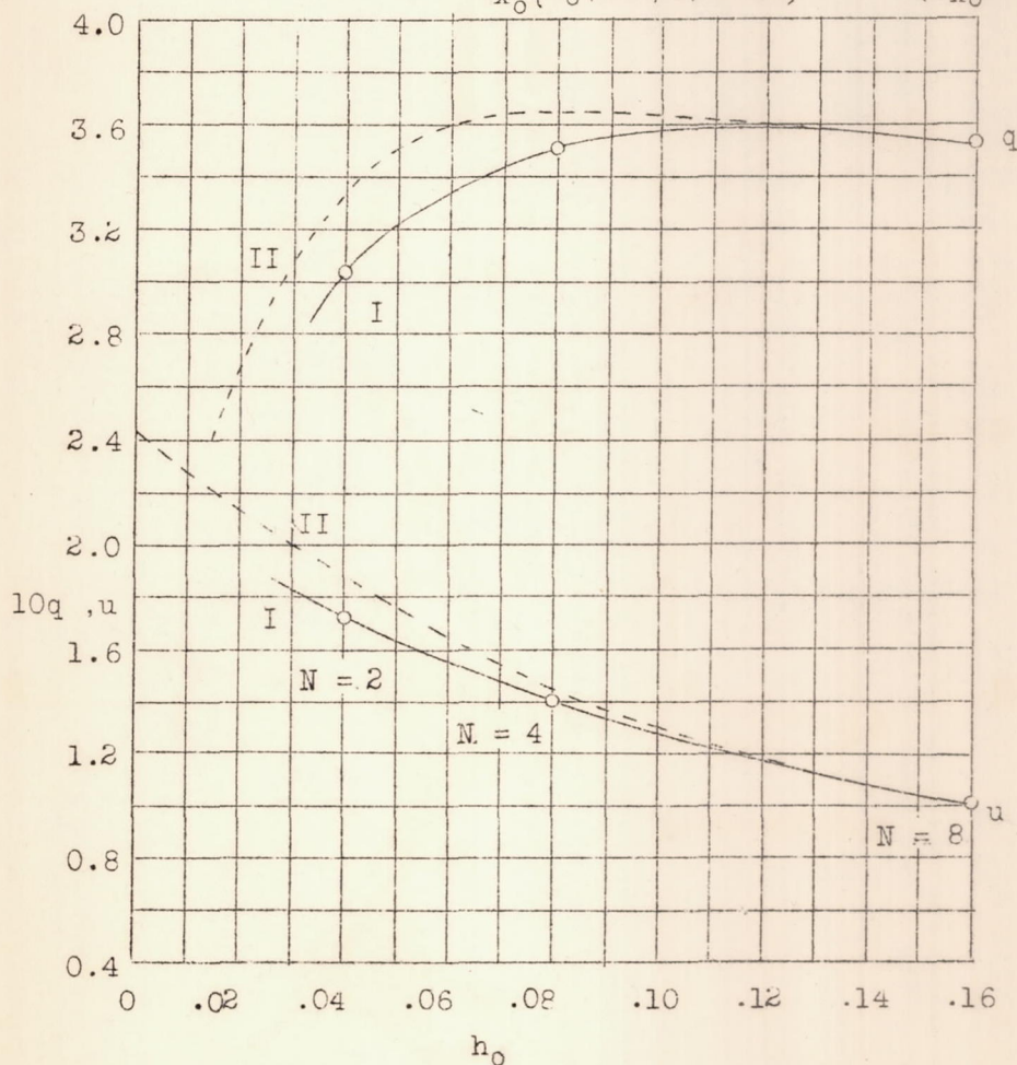
Figure 8.- Lifting quality q and inherent quality u of blades of total area s plotted against solidity ratio h_0 \frac{s}{\pi D^2/4} (near ground \delta=1 ).
