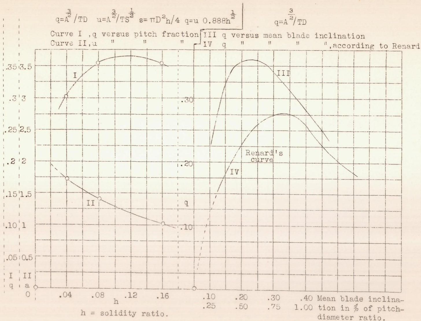
Figure 3.- Test data obtained in 1907 with the balance, Fig.2.
