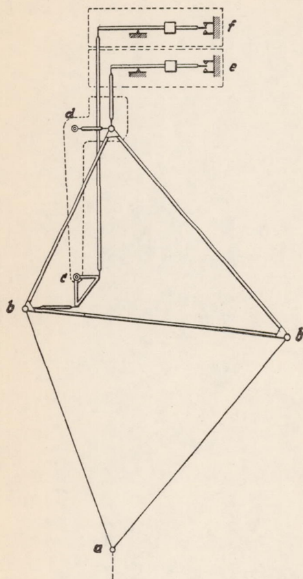
Figure 9.- Force decomposers.
