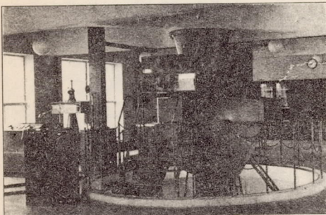
Figure 6.- Test room with six-component balance.
