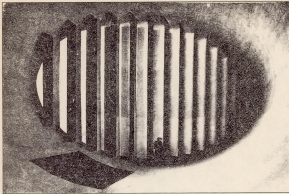
Figure 4.- Guides with vent aft of diffuser.
