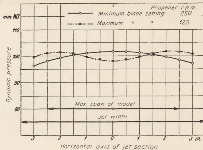
Figure 10.- Dynamic pressure curve on the horizontal axis of the jet section for extreme propeller-blade setting.
