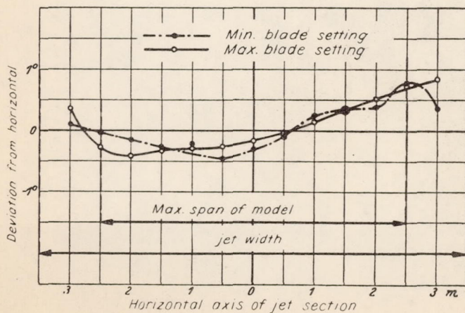
Figure 12.- Direction curve on horizontal axis of jet section for extreme propeller-blade setting.
