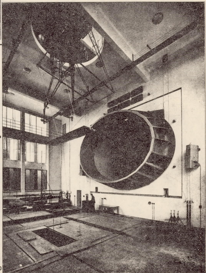
Figure 7.- View of entrance cone, and suspended model airfoil.
