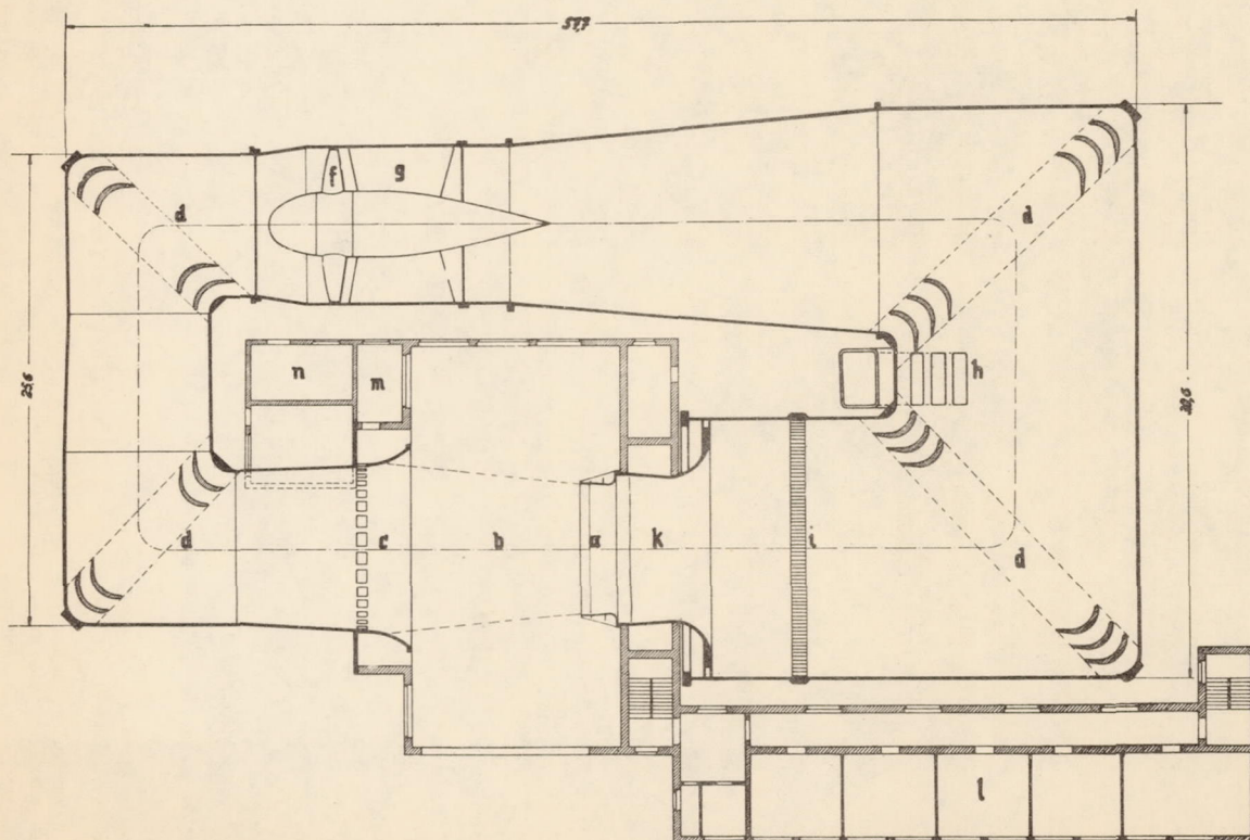
Figure 3.- Cross section of tunnel at level of tunnel axis.
