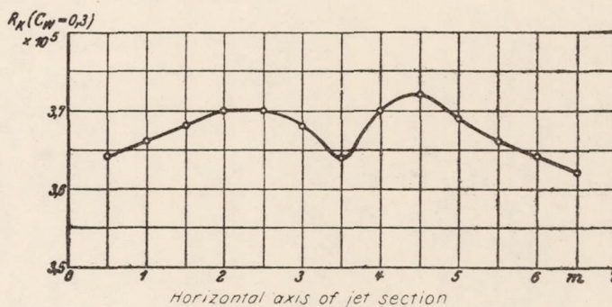
Figure 11.- Jet turbulence investigation; R_k(c_w=0.3) on the long axis of the jet section.
