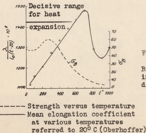
Figure 8.- Steel with 0.22% C content.
