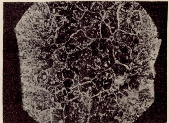
Figure 9.- Overheat zone of a very susceptible carbon steel with its peculiar ferrite spots.
