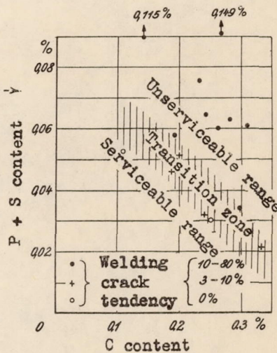
Figure 10.- Effect of C and (P+S) content on the welding crack tendency of non-alloyed steel.
