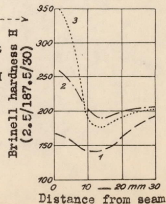
Figure 11.- Effect of Brinell hardness H in welds of different steels.
