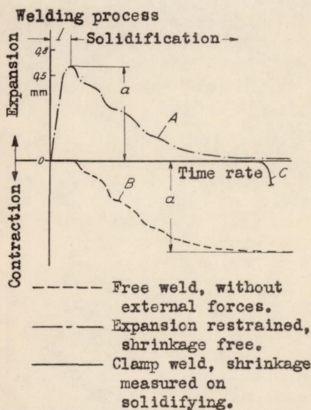
Figure 5.- Elongation - shrinkage stresses on a small specimen (qualitative only).
