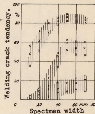
Figure 7.- Effect of specimen width in the clamp weld test, on three sheets of varying degrees of weld cracking tendencies.
