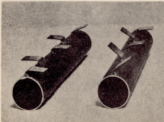
Figure 12.- Bending test.
