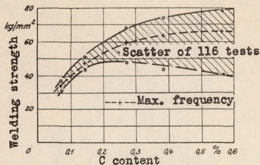
Figure 1.- Welding resistance of steels of varying C content.
