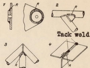
Figure 2.- Illustrations of welds with welding cracks R
