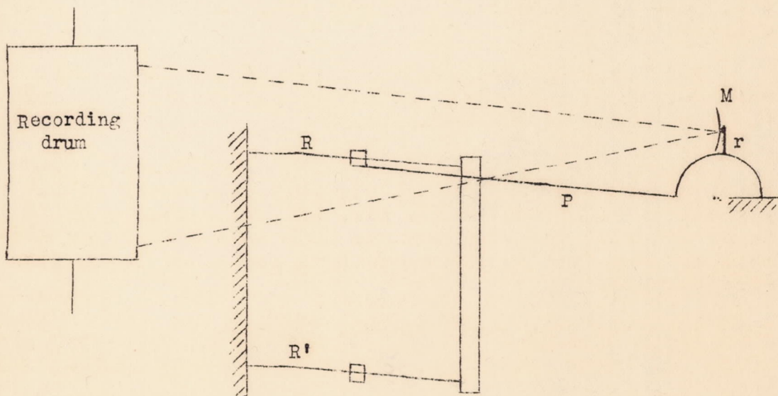
Figure 2.- Parallelogram balance.
