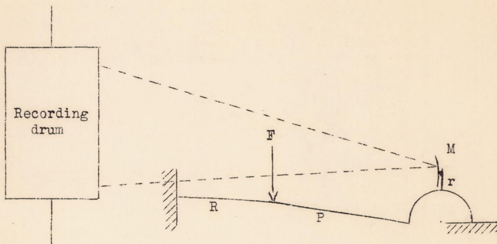
Figure 1.- Simple balance.
