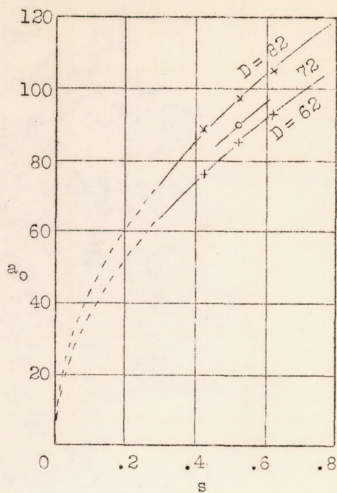
Figure 12.- Optimum hole spacing a_o versus sheet thickness s .
