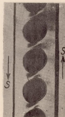
Figure 9.- Sheet distorted in shear showing torn flanging.
