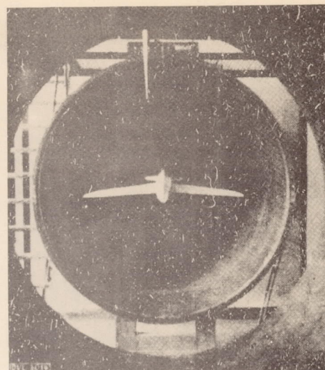
Figure 3.- Suspension of flying-boat model, looking through entrance cone toward exit cone.
