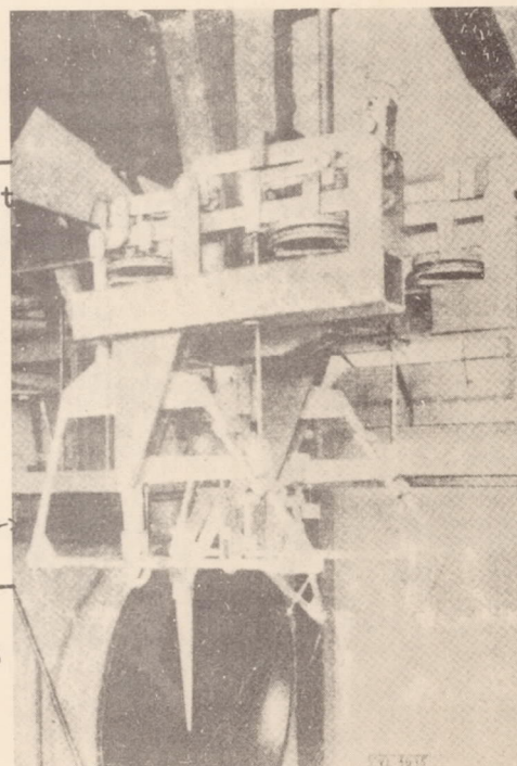
Figure 4.- Six-component balance.
