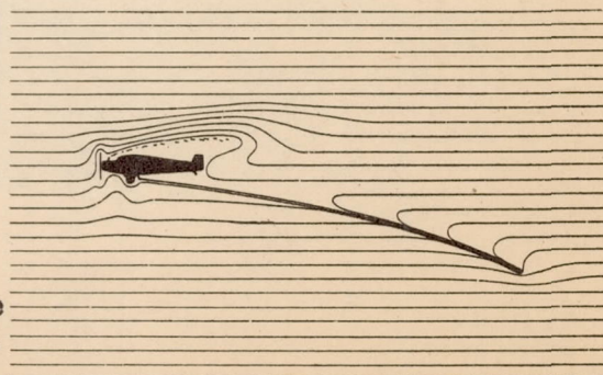
Figure 5.- Airplane with antenna in electric field.
