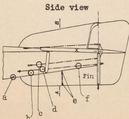
Figure 9.-Damage to a wood-fabric airplane
