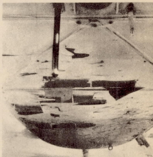
Figure 16.- Destruction of fuselage covering due to pressure effect.
