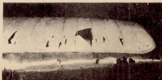
Figure 21.- Damage to glider due to hail.
