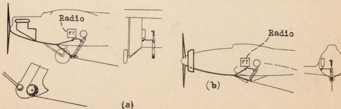
Figure 20.- Lightning protection for airplanes with retractable landing gear.
