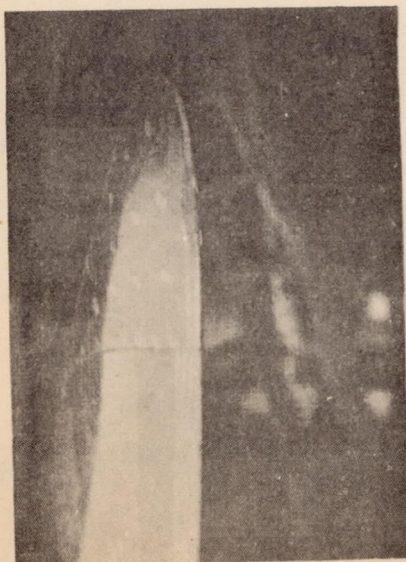
Figure 11. Metal tipping damaged at trailing edge of propeller.
