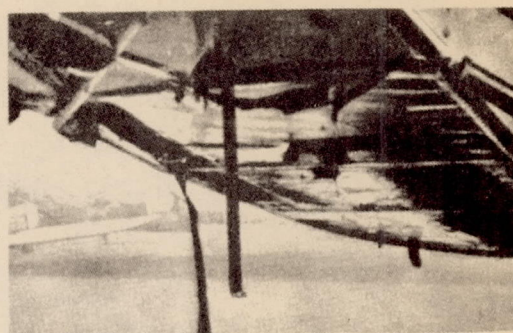
Figure 15.- Destruction of fuselage covering due to pressure effect (according to L'illustration 10/24/31)
