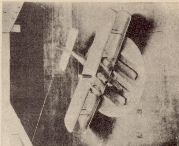
Figure 1.- Model suspended in wind tunnel over plate representing surface of water.
