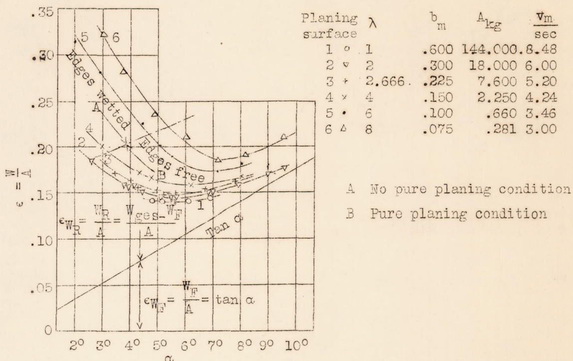
Figure 3.- Planing number \epsilon plotted against angle of trim \alpha .
