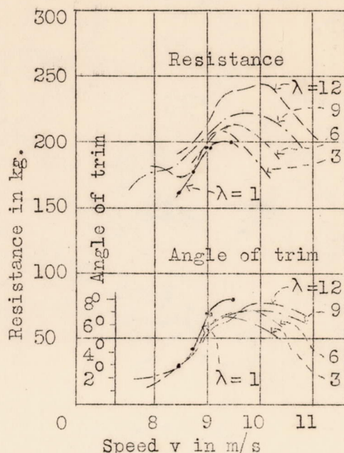
Figure 7a.- Resistance and angle of trim of full-scale float for M_2 = \text{constant} , along with resistances and angles of attack converted to full scale for \lambda = 3, 6, 9, 12 with same moment.
