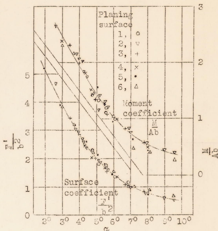
Figure 5.- Surface coefficient F'/b^2 and moment coefficient M/Ab plotted against \alpha .
