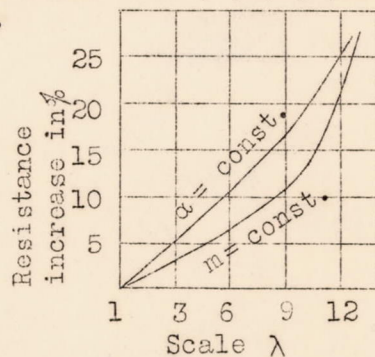
Figure 7a.- Resistance and angle of trim of full-scale float for M_2 = \text{constant} , along with resistances and angles of attack converted to full scale for \lambda = 3, 6, 9, 12 with same moment.
