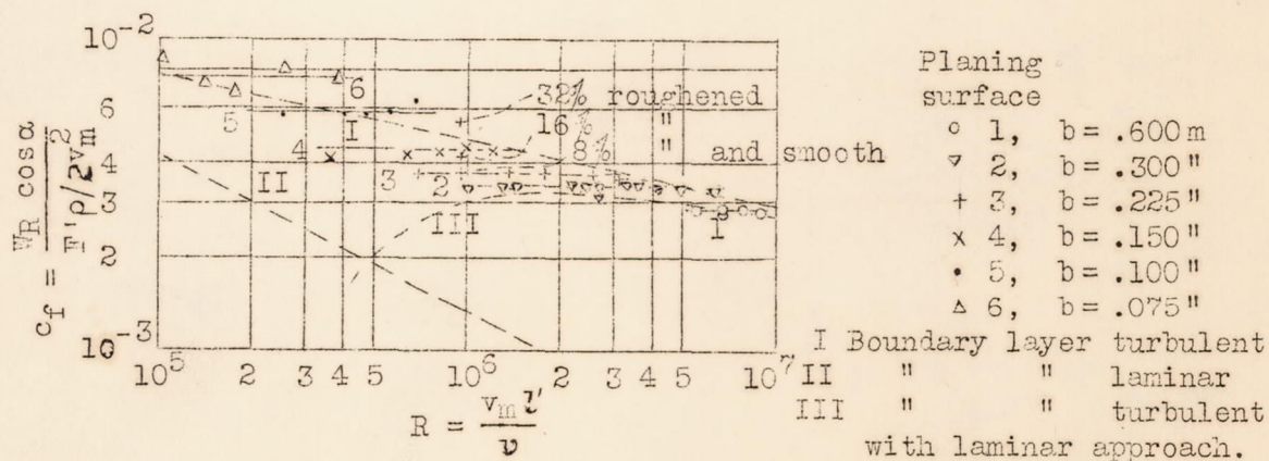
Figure 4.- Coefficient of frictional resistance plotted against Reynolds Number for flat planing surfaces.
