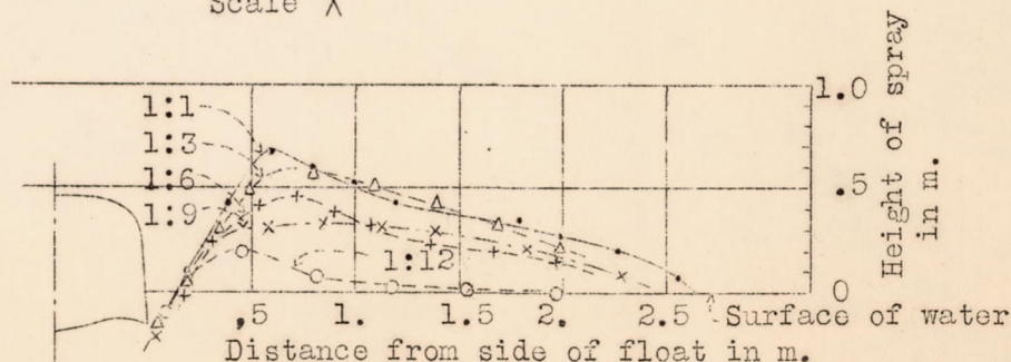
Figure 9.- Spray formation measured on full-scale float 0.5 m (1.64 ft.) in front of step at v = 8.75 \text{ m/s} (28.7 ft./sec.) and on all models at same distance and at corresponding speeds, converted to full-scale.
