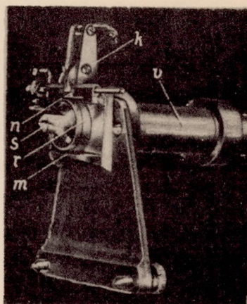
Figure 4.- Test apparatus with reflecting extensometer.
