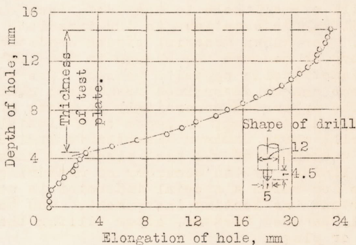
Figure 2.- Depth against elongation of hole (mm).
