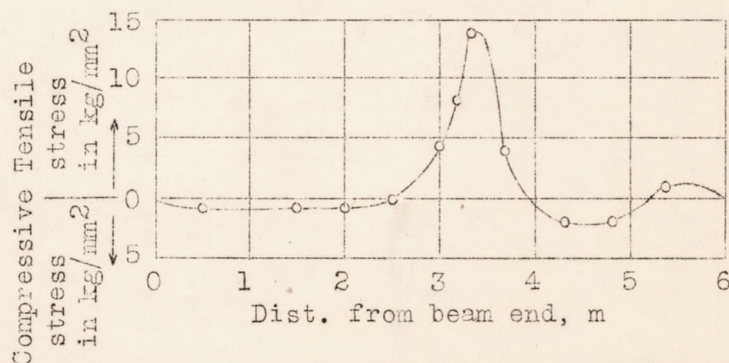
Figure 9.- Distribution of inherent stresses over length of channel NP 26, measured in middle of web.
