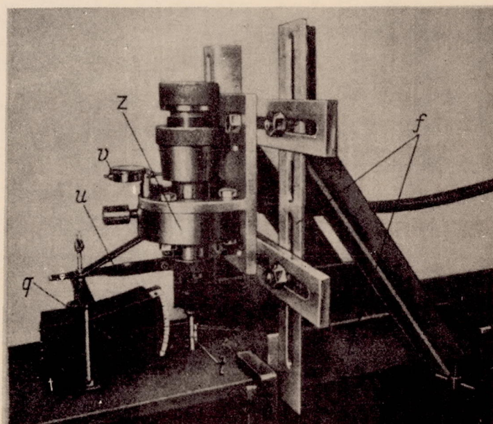
Figure 5.- Apparatus for using indicator.
