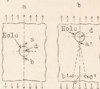
Figure 1.- Arrangement of reflecting and indicating instruments for measuring hole deformations.
