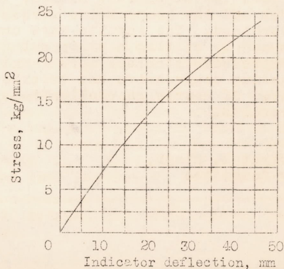
Figure 3.- Calibration curve for a soft steel.
