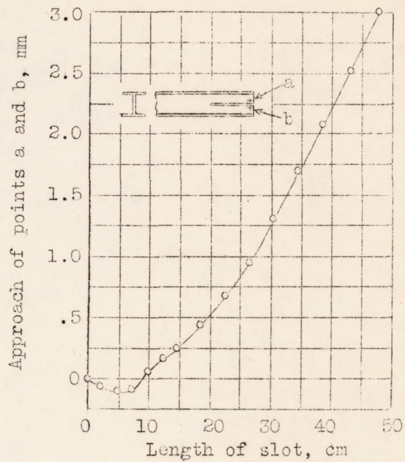
Figure 10.- Approach of points a and b due to slot in web middle at right end of H beam II.
