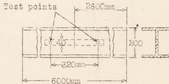
Figure 11.- Location and shape of test strip in H beam I.
