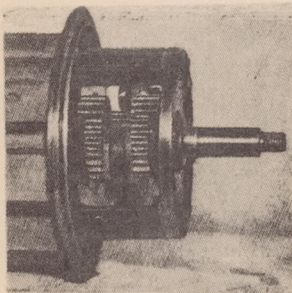
Fig.20 Driving gear.
