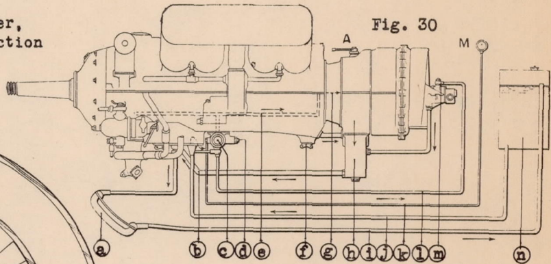
Fig.30, 31 Oil and fuel systems on Farman 12 WE engine with supercharger.
