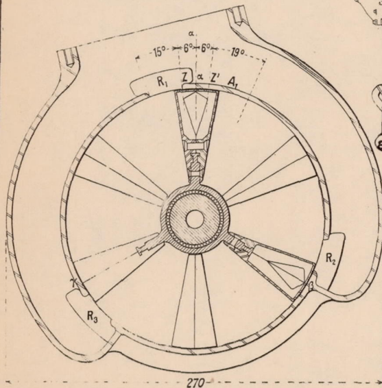
Fig. 23 P.Z. supercharger, transverse section showing two 3-blade systems
