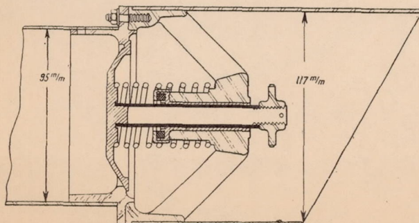
Fig. 29 Valve on manifold
