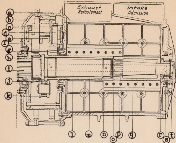
Fig. 22 P.Z. supercharger, longitudinal section
