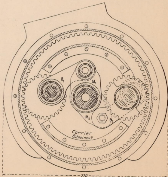
Fig. 24 P.Z .supercharger,transverse section showing driving gear of coaxial shafts
