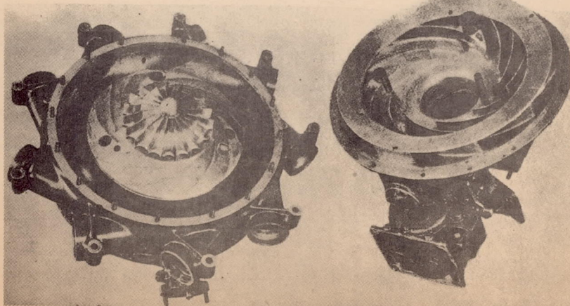
Fig. 28 Pratt & Whitney supercharger (on "Wasp" engine)
