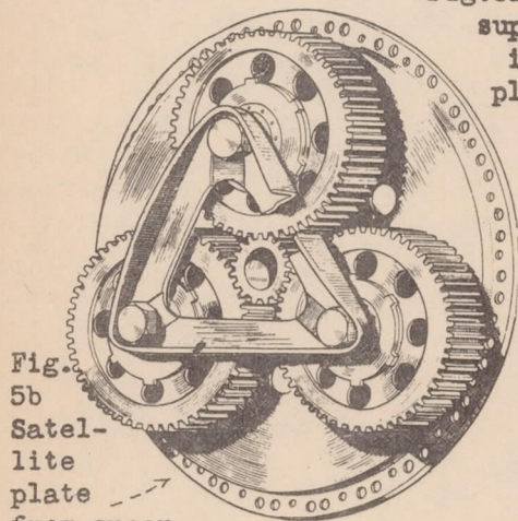
Fig. 5, Farman mechanical control of Rateau supercharger. (In reality this supercharger has two stages)
