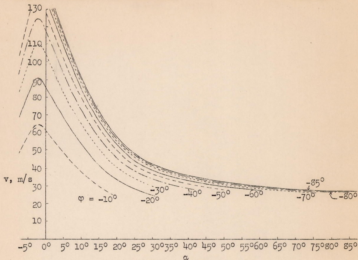
Fig.15 Path velocity against \alpha and \phi .
