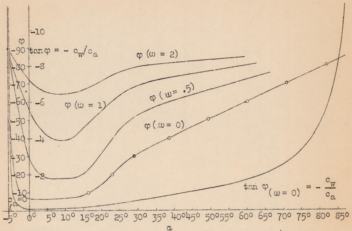
Fig. 17 Angle of glide \varphi ( \omega = \text{const.} ) and \tan \varphi(\omega = 0) = -\frac{c_a}{c_w} against \alpha and rate of rotation.
