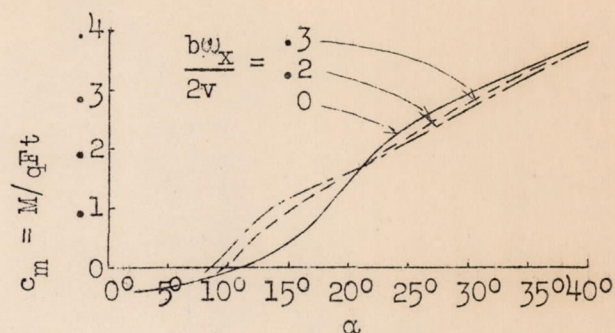
Fig.13 Aerodynamic moment about lateral axis against \alpha and against rotation \omega_x about path axis (Reference 7).
