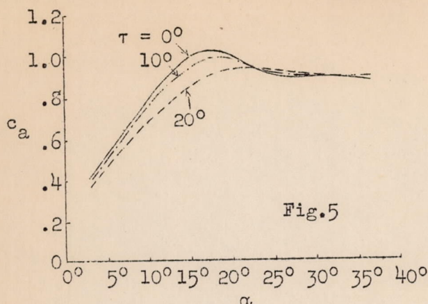
Figs. 5, 6 Lift and drag plotted against \alpha and \varphi . (Reference 6)
