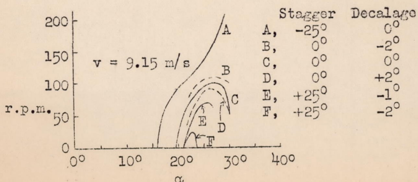
Fig. 34 Balance of moments about path axis of a biplane; rate of rotation about path axis plotted against \alpha , stagger and decalage. (Reference 9)
