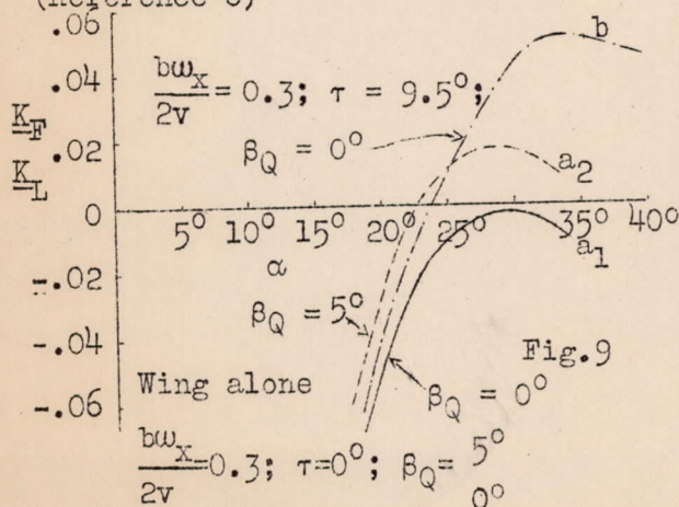
Figs. 9, 10 Aerodynamic moment about longitudinal and normal axis plotted against \alpha and \tau , as well as against w_x about path axis and aileron displacement \beta_Q , (Reference 8 and 4).
