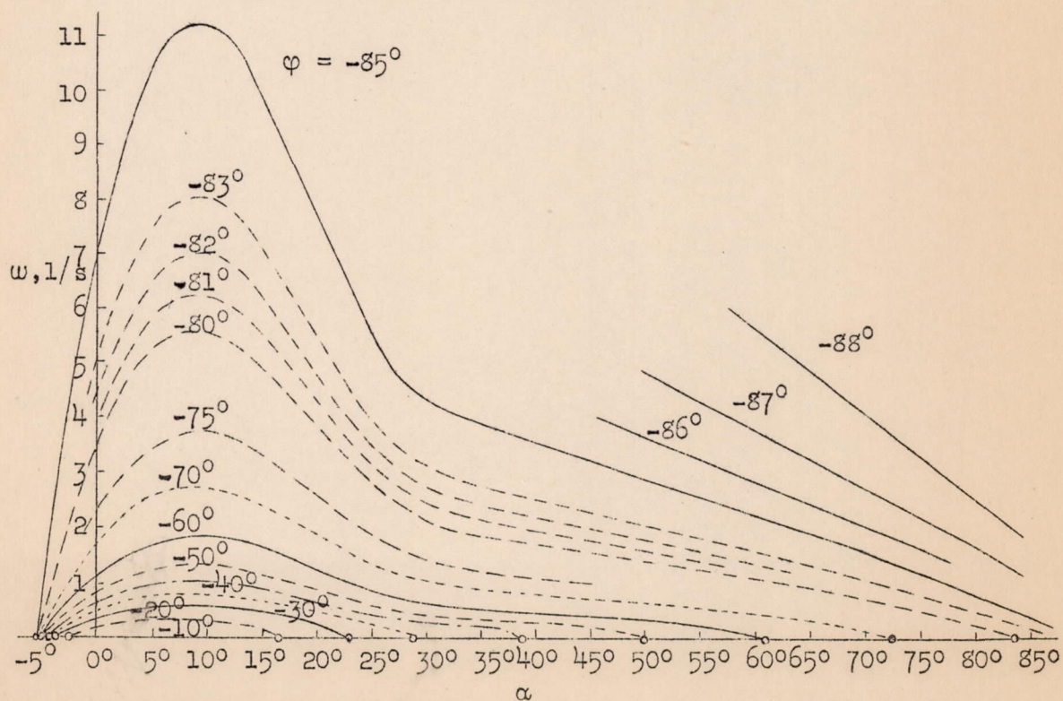
Fig.16 Rate of rotation against \alpha and \phi .
