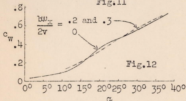
Figs.11,12 Lift and drag against \alpha and rotation \omega_x about path axis (Reference 4).
