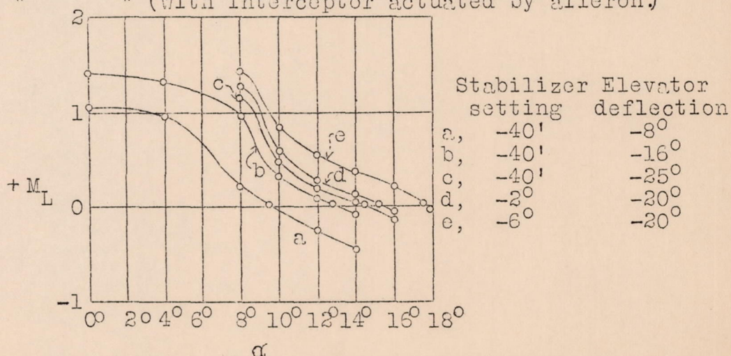
Fig.17 Longitudinal moments determined in the wind tunnel for the model of a well known airplane with cantilever wings at various angles of setting of the stabilizer and elevator.
