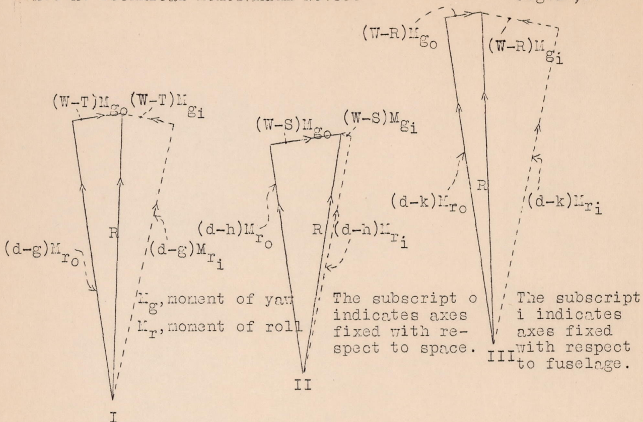
Fig.16 Comparison of resultant moment vectors for three different arrangements.
