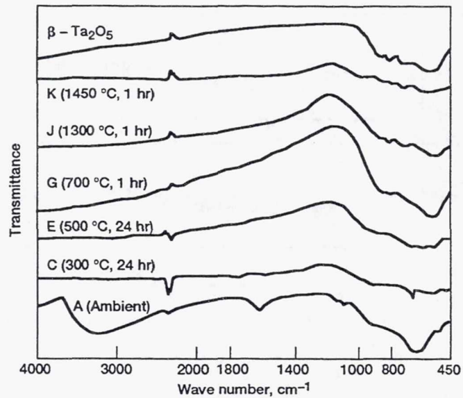
Figure 7.—Infrared absorption spectra of tantalum pentoxide gel fired under various conditions as given in Table II.
