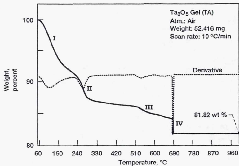
Figure 4.—A typical TGA curve recorded at a scan rate of 10 °C/min in air and its derivative for room temperature dried tantalum pentoxide gel.
