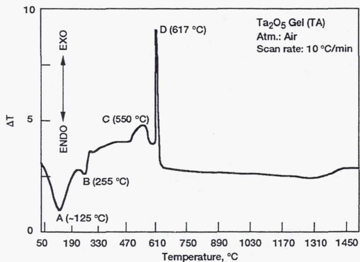
Figure 3.—A typical DTA thermogram recorded at a heating rate of 10 °C/min in air for room temperature dried tantalum pentoxide gel.
