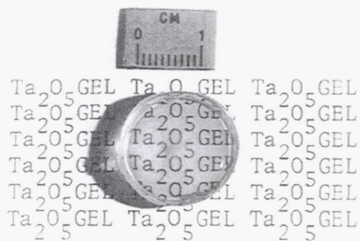
Figure 1.—Photograph showing a typical transparent monolithic ~1.2 cm diameter disc of dry tantalum oxide gel.
