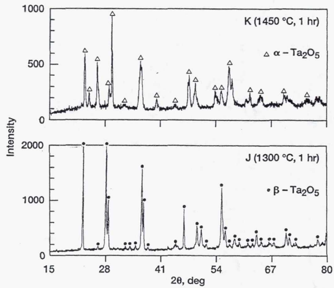
Figure 6.—Powder X-ray diffraction patterns of tantalum pentoxide gel pyrolyzed to various temperatures (Table II).
