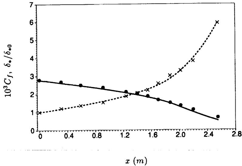
FIGURE 2. Friction coefficient (•) and displacement thickness (x) versus downstream distance for the Samuel and Joubert experiment. Curves are solution of model, symbols experimental data.
