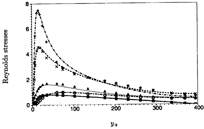
FIGURE 1. Comparison of model (lines) to DNS (symbols) profiles of Reynolds stresses in channel flow at R_\tau = 395 . +, \overline{u^2} ; x, k ; \Delta , \overline{w^2} ; o, \overline{v^2} ; ■, -\overline{uv} .
