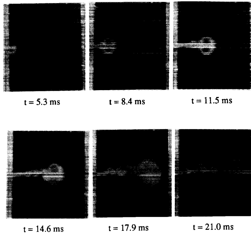
FIGURE 4. Sequence of photographs showing the vortex pair evolution without cross-flow. Slot width = 3 mm. Time t = 0 ms corresponds to the speaker excitation.
