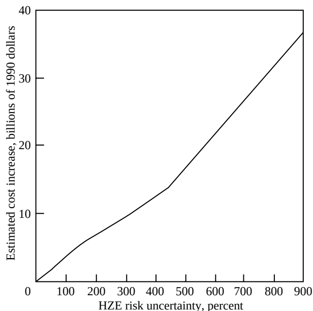
Figure 27. Excess mission cost from added shielding for vehicle and habitat to ensure astronaut safety for 29-month Mars mission.
