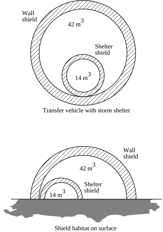
Figure 12. Models used for transfer vehicle and habitat configurations.
