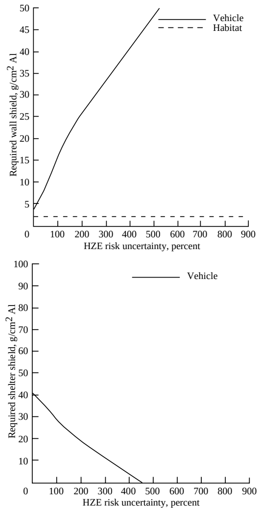
Figure 26. Required shield for walls and shelters to protect astronauts from SEP for 29-month mission to Mars.
