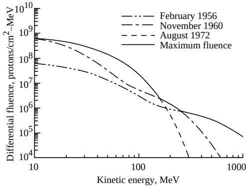
Figure 11. An estimate for the maximum fluence spectrum for an SEP event.
