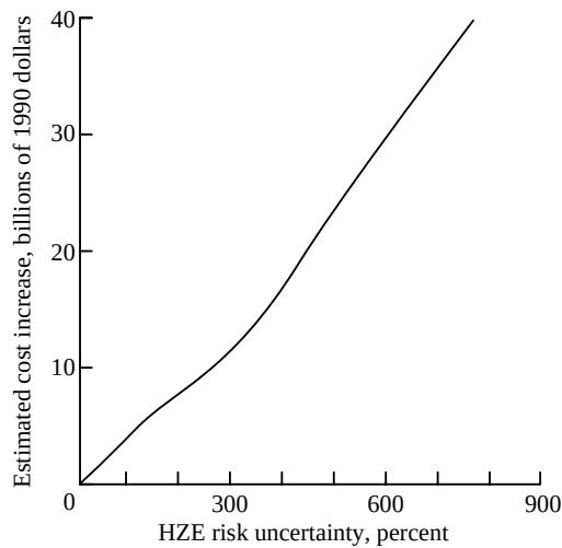
Figure 24. Excess mission cost from added shielding for vehicle and habitat to ensure astronaut safety for 18-month Mars mission.
