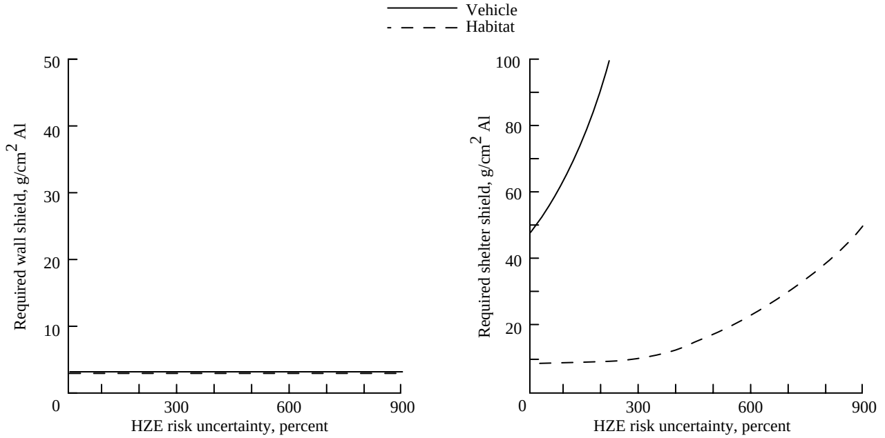
Figure 15. Required shield for walls and shelters to protect astronauts from SEP for 60-day lunar mission.
