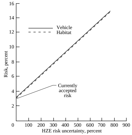
Figure 25. Excess fatal cancer risk for astronauts exposed to SEP in vehicles or habitats for 29-month Mars mission nominal design.
