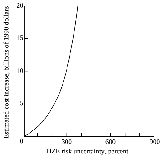
Figure 20. Excess mission cost from added shielding for vehicle and habitat to ensure astronaut safety for 6-month lunar mission.
