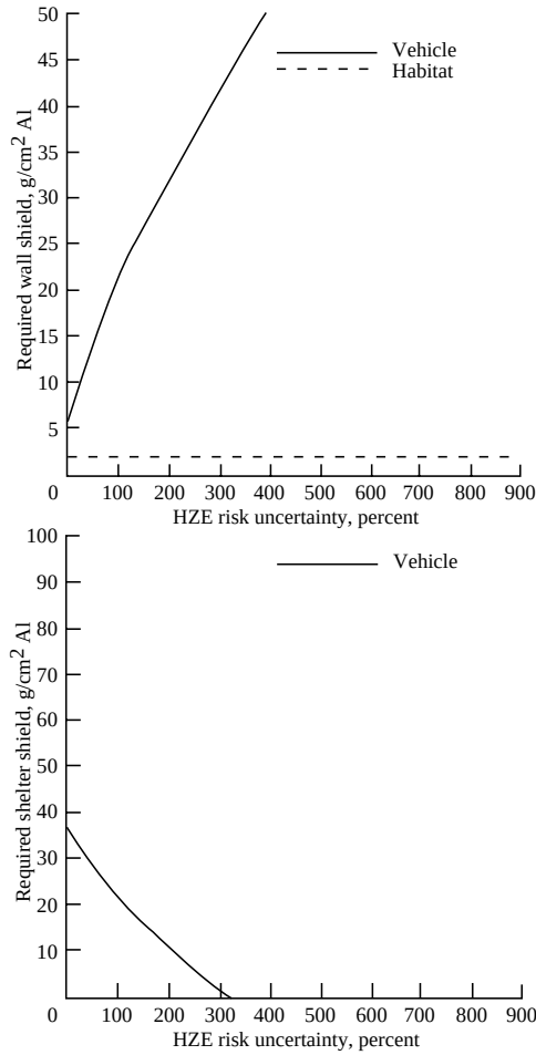
Figure 23. Required shield for walls and shelters to protect astronauts from SEP for 18-month mission to Mars.
