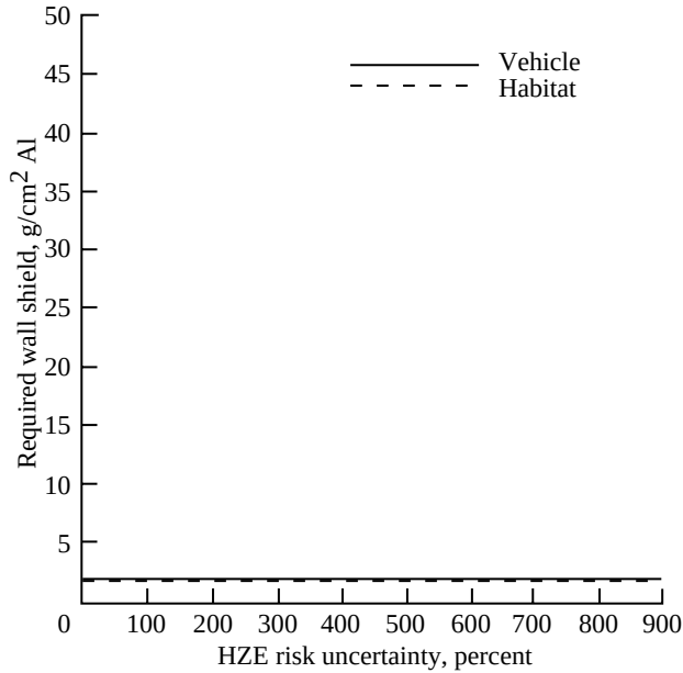
Figure 19. Required shield for walls and shelters to protect astronauts from SEP for 6-month lunar mission.
