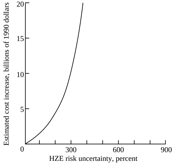
Figure 16. Excess mission cost from added shielding for vehicle and habitat to ensure astronaut safety for 60-day lunar mission.
