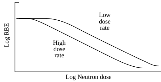
Figure 8. Schematic of RBE for neutron exposure at different dose rates.
