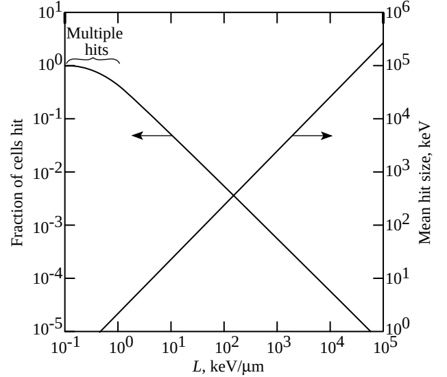
Figure 6. Nonuniformity of exposure at the 1-Gy level for a typical tissue system. D = 1 \text{ Gy} ; \sigma_g \approx 100 \mu\text{m}^2 .
