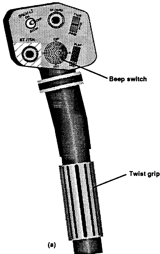
Figure 3. Location of auxiliary thrust control inceptors. (a) collective grip; (b) cyclic grip
