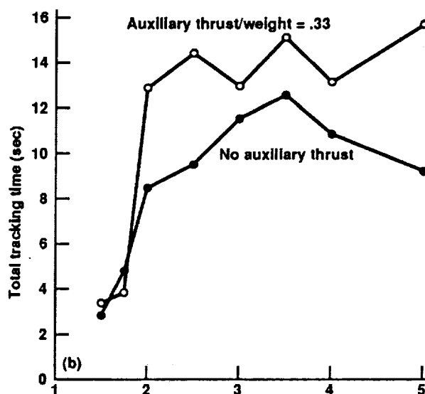
Figure 19. Air-to-air task results with and without auxiliary thrust. (a) mean CHRs for both tasks; (b) task performance for the mountain air-to-air task.
