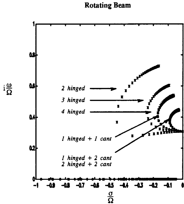
Figure 7 Modal Solutions For Beam Equations
