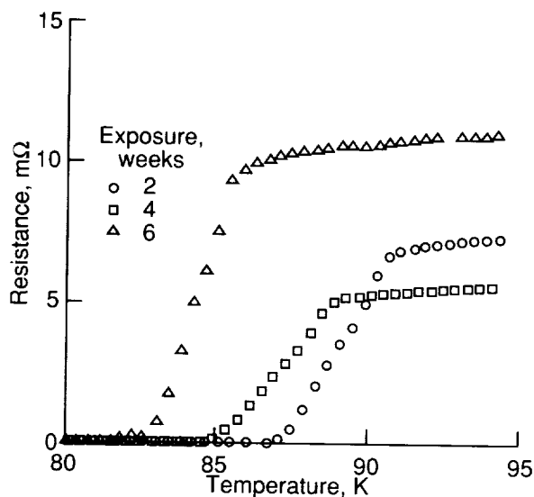
Figure 11. Resistance-versus-temperature plot of superconducting specimens aged at 81 percent relative humidity.
