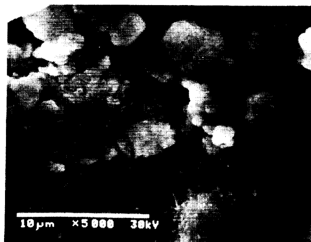
Figure 5. SEM micrograph showing formation of small, needle-like grains (bottom right) on surface of YBa 2 Cu 3 O 7-x specimen stored at 66 percent relative humidity for 6 weeks.
