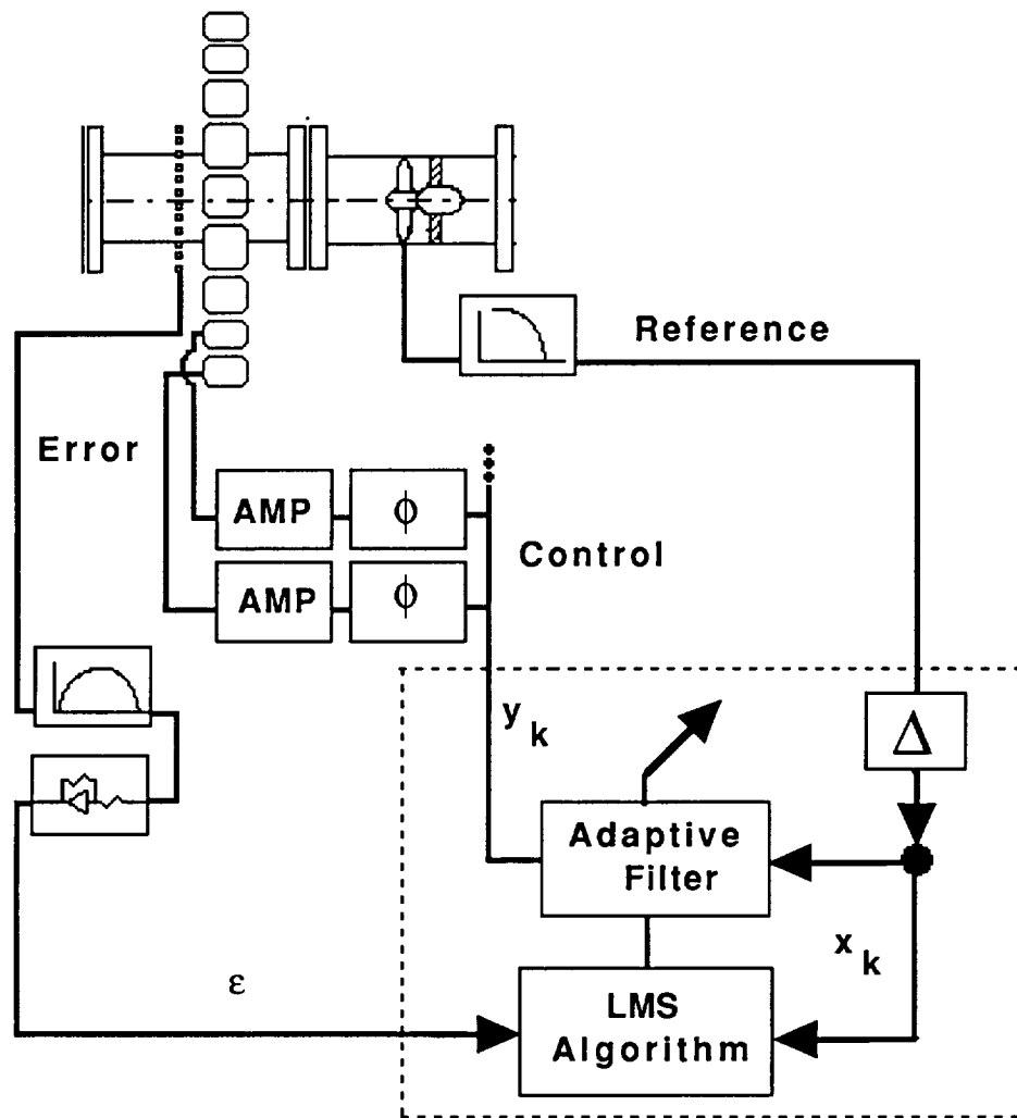
Figure 6. Fan noise control system setup
