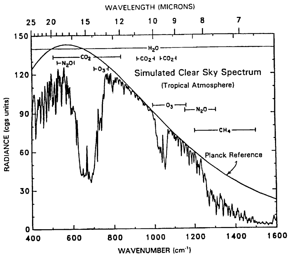
Fig. 10.1. Clear sky spectrum at 3 cm -1 (IRIS) resolution. The spectral locations of the principal absorption features are identified.
