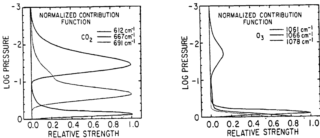
Fig. 10.2. Contribution (weighting) functions illustrating height and wavelength dependence of radiance emission level used in retrieval of height dependent profiles for temperature from the CO 2 band (left) and ozone (right).
