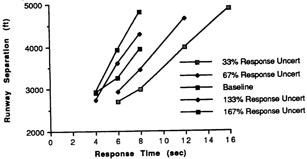
Figure 42. Response Time Uncertainty
