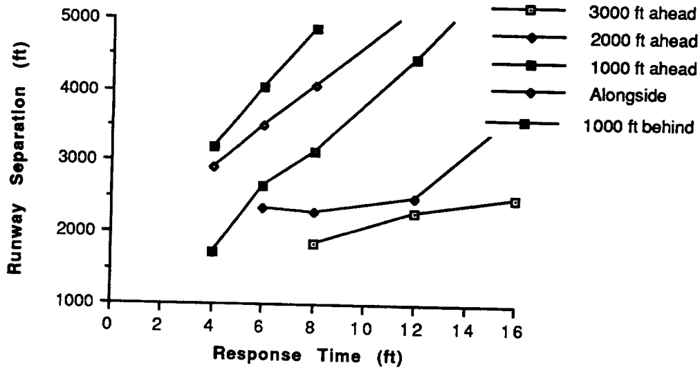
Figure 40 Longitudinal Offset Distance
