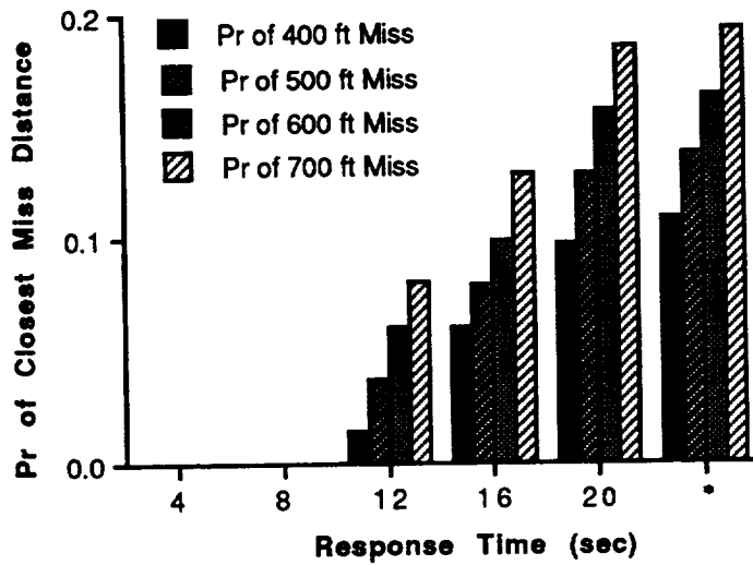
Figure 36 Sensitivity Analysis - Total Response Time
