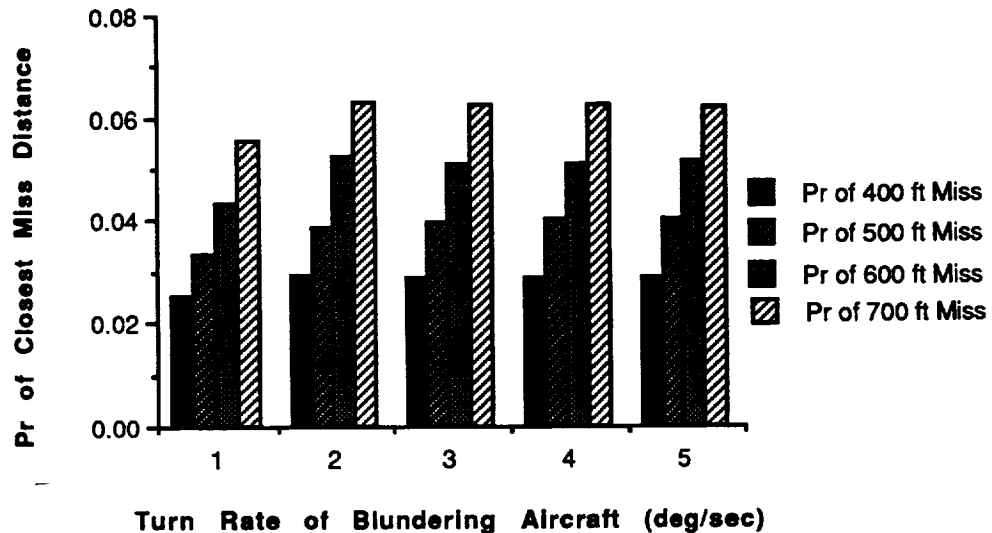
Figure 30. Sensitivity Analysis - Turn Rate of Blunderer
