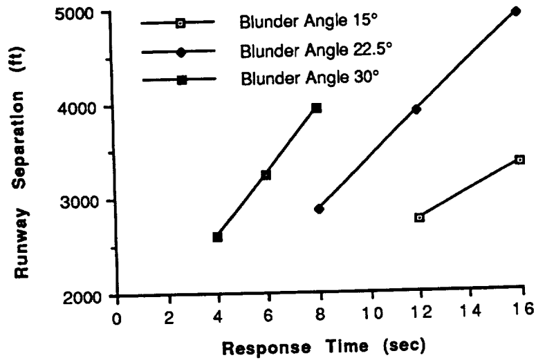
Figure 39 Blunder Angle
