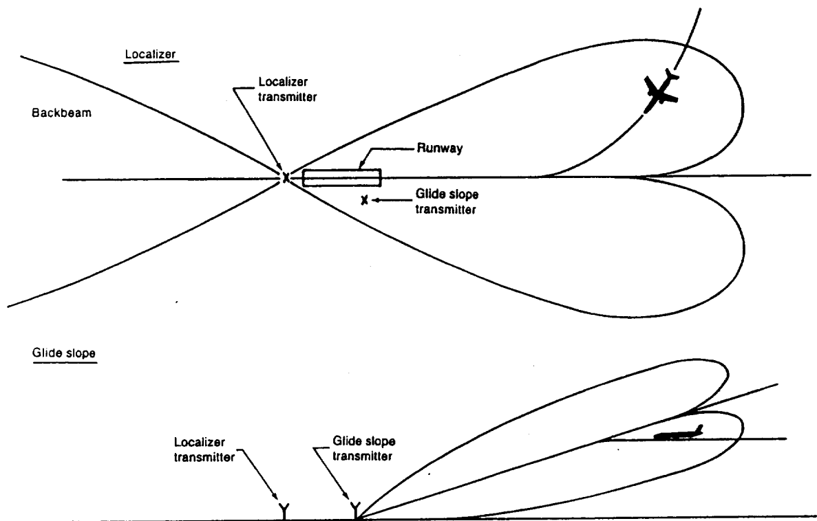
Figure 13. Localizer and Glideslope Geometry of ILS Approach
