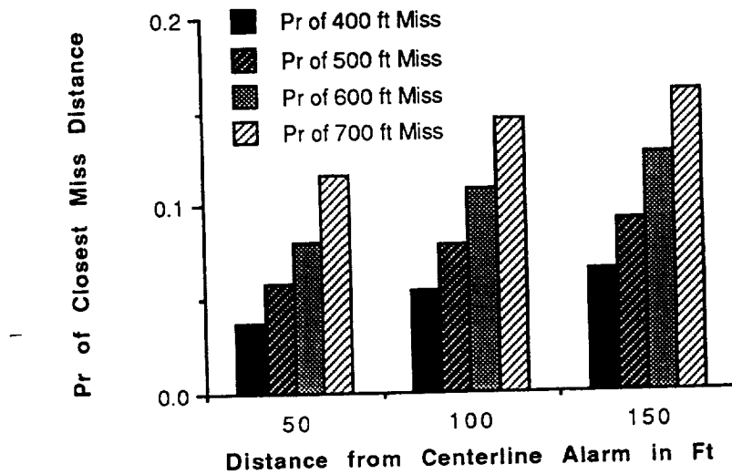
Figure 57. Sensitivity Analysis - Alarm Distance
