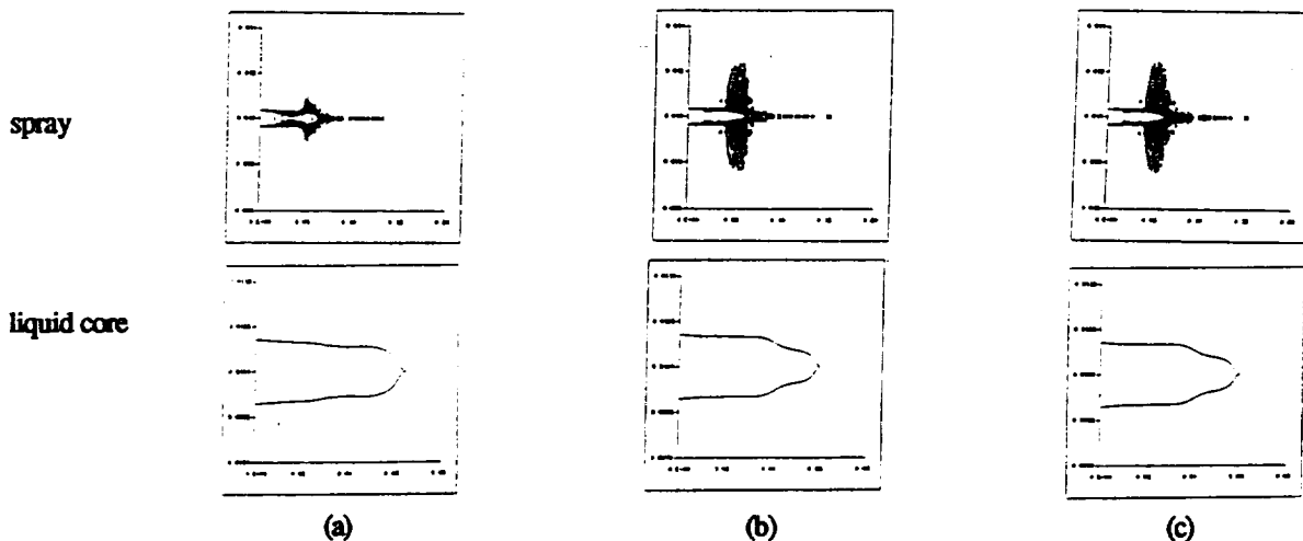
Figure 4. Spray and Associated Liquid Core Profiles for: (a) non-reacting spray; (b) reacting with infinite rate chemistry; and (c) reacting with one step finite rate model
