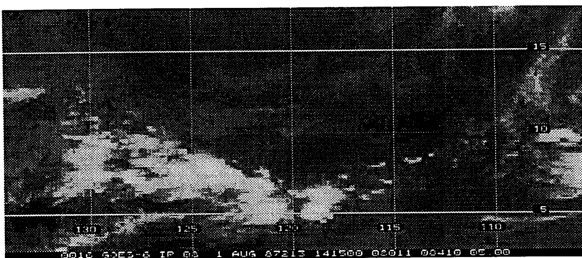
Fig. 1. GOES-W IR image of ITCZ on 1 Aug 87.
