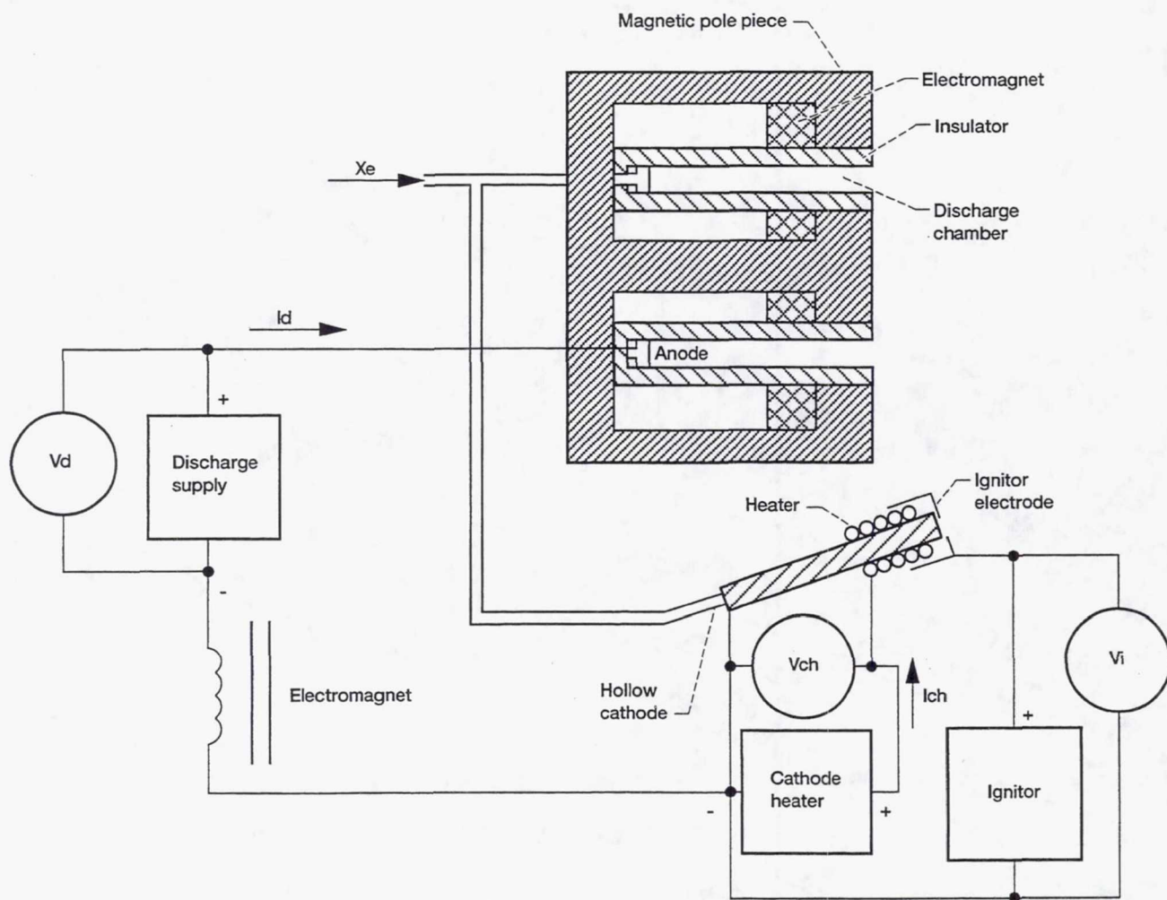
Figure 4.—Electrical schematic of test set-up. (From Ref. 7).
