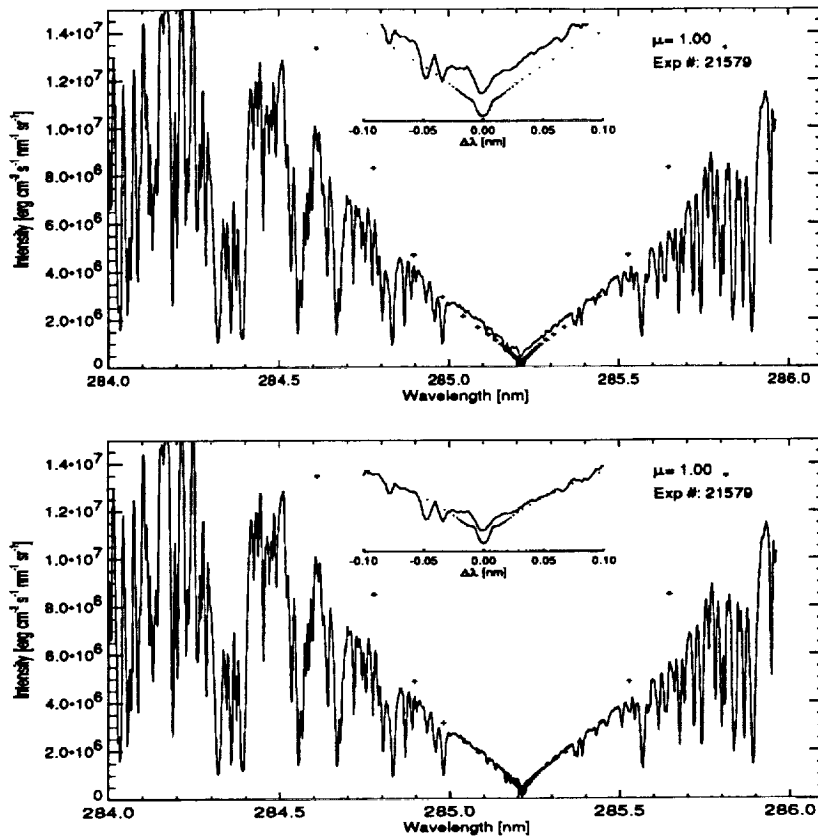
Figure 3: Comparison of the theoretical line profile of the \text{Mg I } \lambda 285.21 \text{ nm} line from FAL models A (plus signs, upper panel) and C (lower panel) with the observed spectrum from UVSP experiment 21579 (solid line). Each panel separately displays the inner two Ångström in the core of the line where the theoretical profiles are represented by dotted curves.
