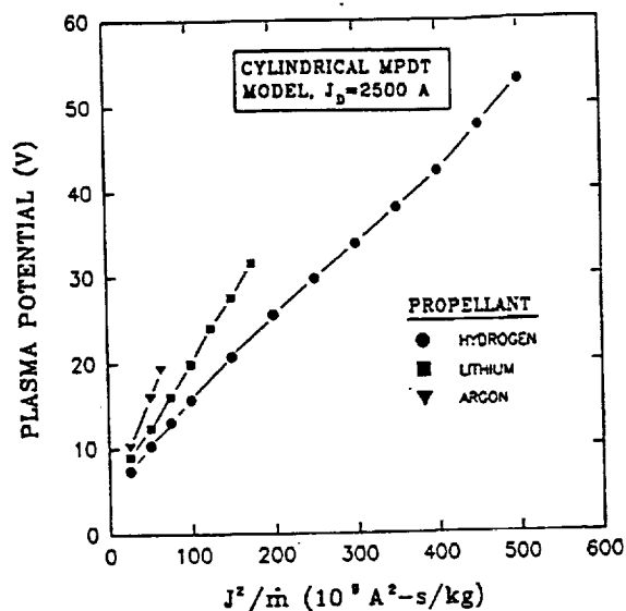
Figure 11. Predicted plasma potential for a simulated 100-kW class cylindrical, self-field MPD thruster operated with hydrogen, lithium, and argon propellants at a constant discharge current of 2500 A.
