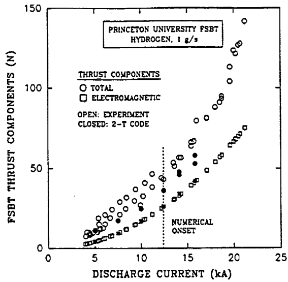
Figure 5. Comparison of measured 28,29 and predicted thrust for the Princeton University full-scale benchmark thruster operated with 1 g/s, hydrogen. Dashed vertical line denotes onset of numerical oscillations.
