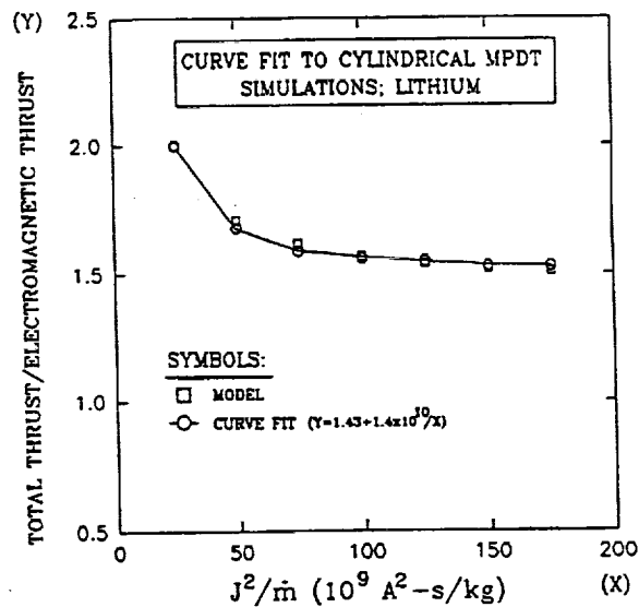
Figure 16. Curve fit to total/electromagnetic thrust as a function of J^2/\dot{m} for a simulated 100-kW class cylindrical, self-field MPD thruster operated with Li.
