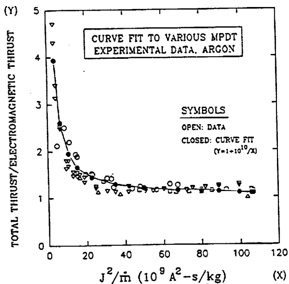
Figure 14. Curve fit to total/electromagnetic thrust as a function of J^2/\dot{m} for the Princeton University full-scale benchmark thruster 27,28 operated at 6 g/s Ar (○) and 3 g/s Ar (□), the Princeton half-scale benchmark thruster 27 operated at 3 g/s Ar (▼), and the Princeton extended anode thruster 41 operated at 6 g/s Ar (△).
