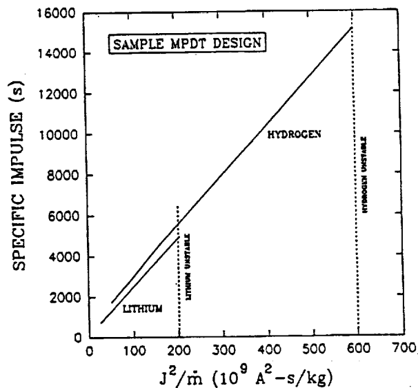
Figure 19. Predicted specific impulse with lithium and hydrogen for the example MPD thruster design. Dashed vertical lines denote predicted limits of stable operation for each propellant.
