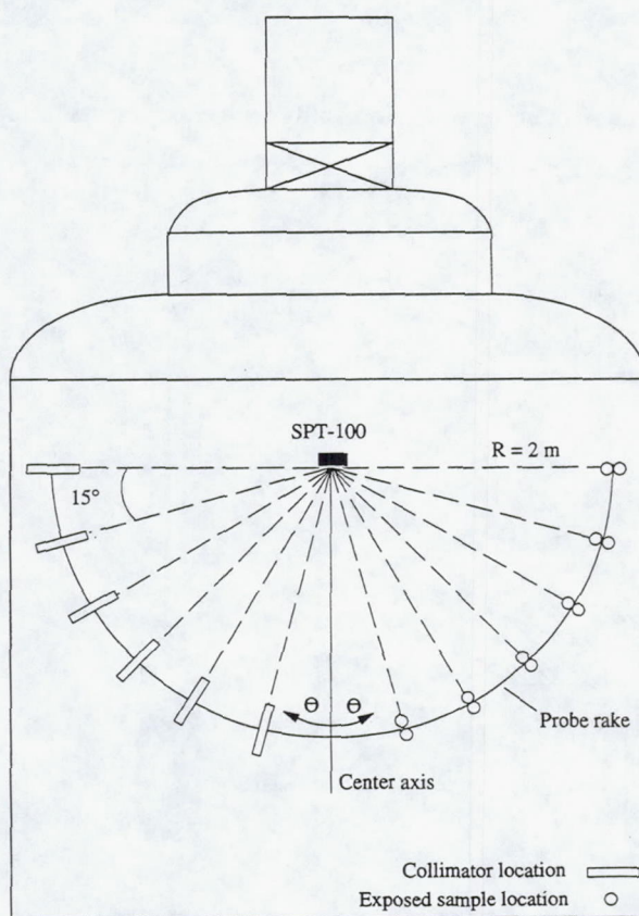
Figure 4 - Schematic of far-field plume probe locations, top view of facility.
