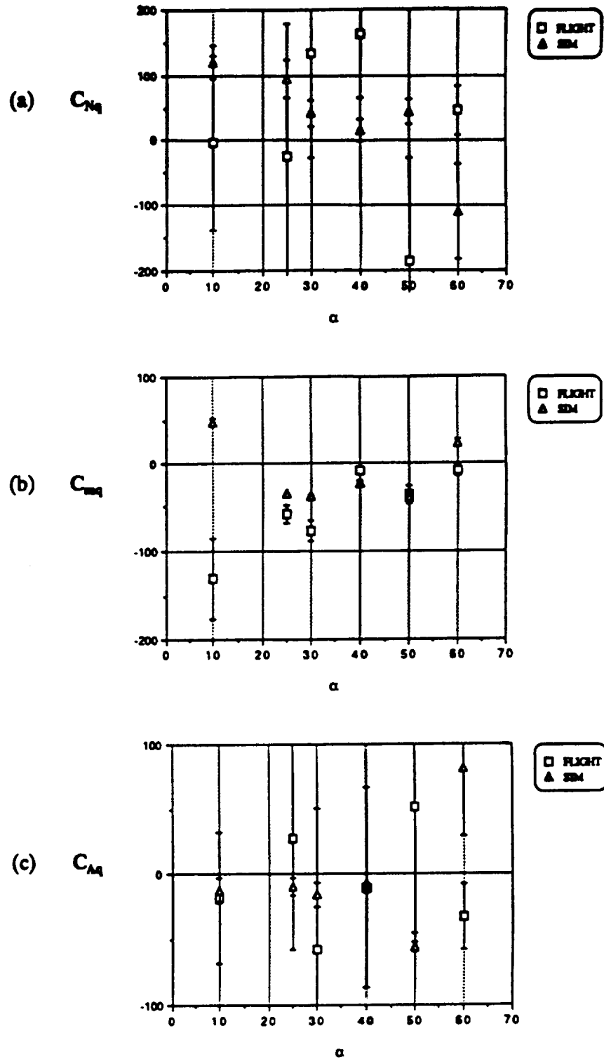
Figure 8.25: Pitch Rate Derivatives (Longitudinal-Directional) (a) Normal Force (b) Pitching Moment (c) Axial Force
