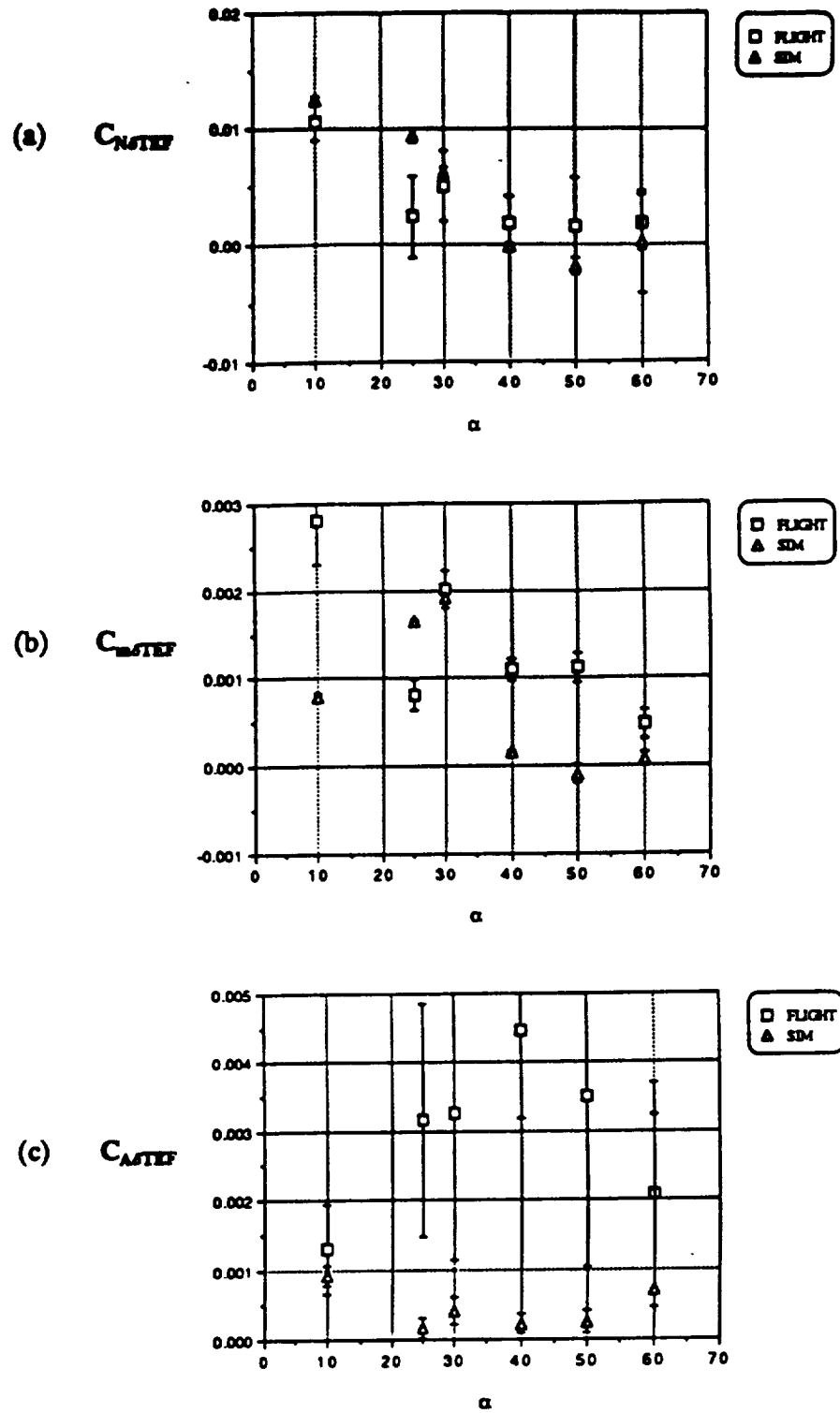
Figure 8.26: Trailing Edge Flap Derivatives (Longitudinal-Directional) (a) Normal Force (b) Pitching Moment (c) Axial Force
