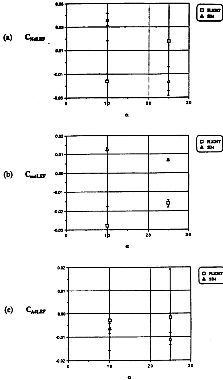
Figure 8.27: Leading Edge Flap Derivatives (Longitudinal-Directional) (a) Normal Force (b) Pitching Moment (c) Axial Force
