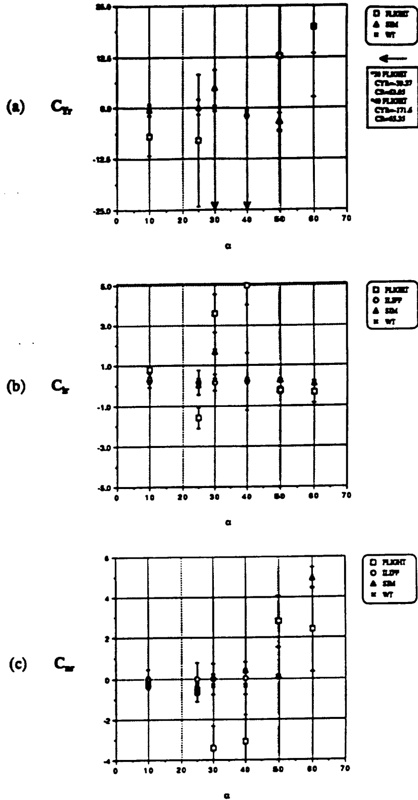
Figure 8.10: Yaw Rate Derivatives (Lateral-Directional) (a) Lateral Force (b) Rolling Moment (c) Yawing Moment
