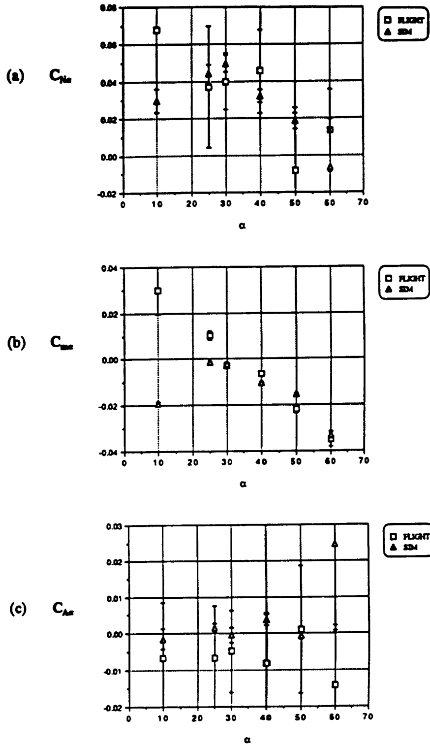
Figure 8.24: Angle of attack Derivatives (Longitudinal-Directional) (a) Normal Force (b) Pitching Moment (c) Axial Force
