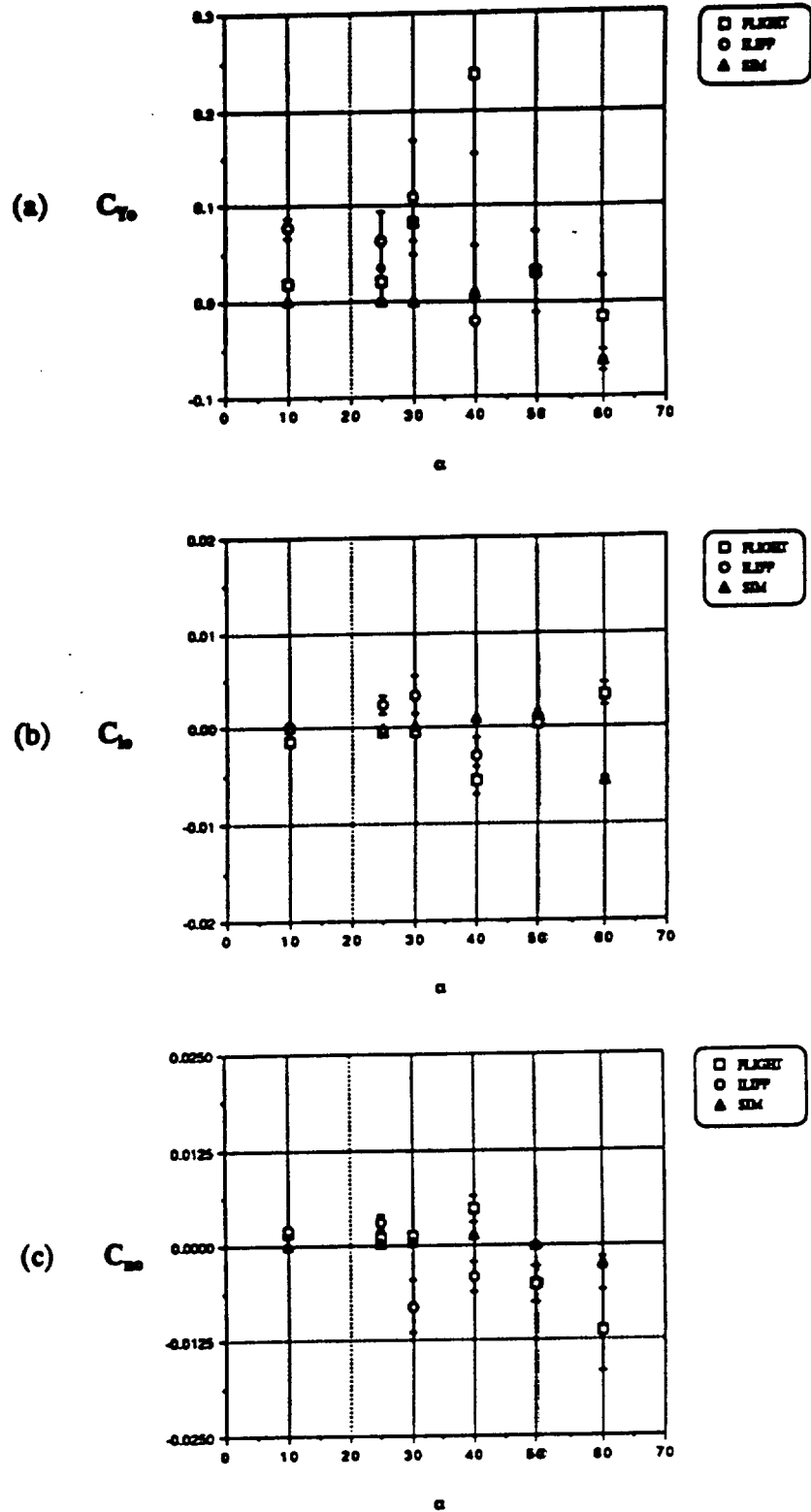
Figure 8.7: Aerodynamic Bias Derivatives (Lateral-Directional) (a) Lateral Force (b) Rolling Moment (c) Yawing Moment
