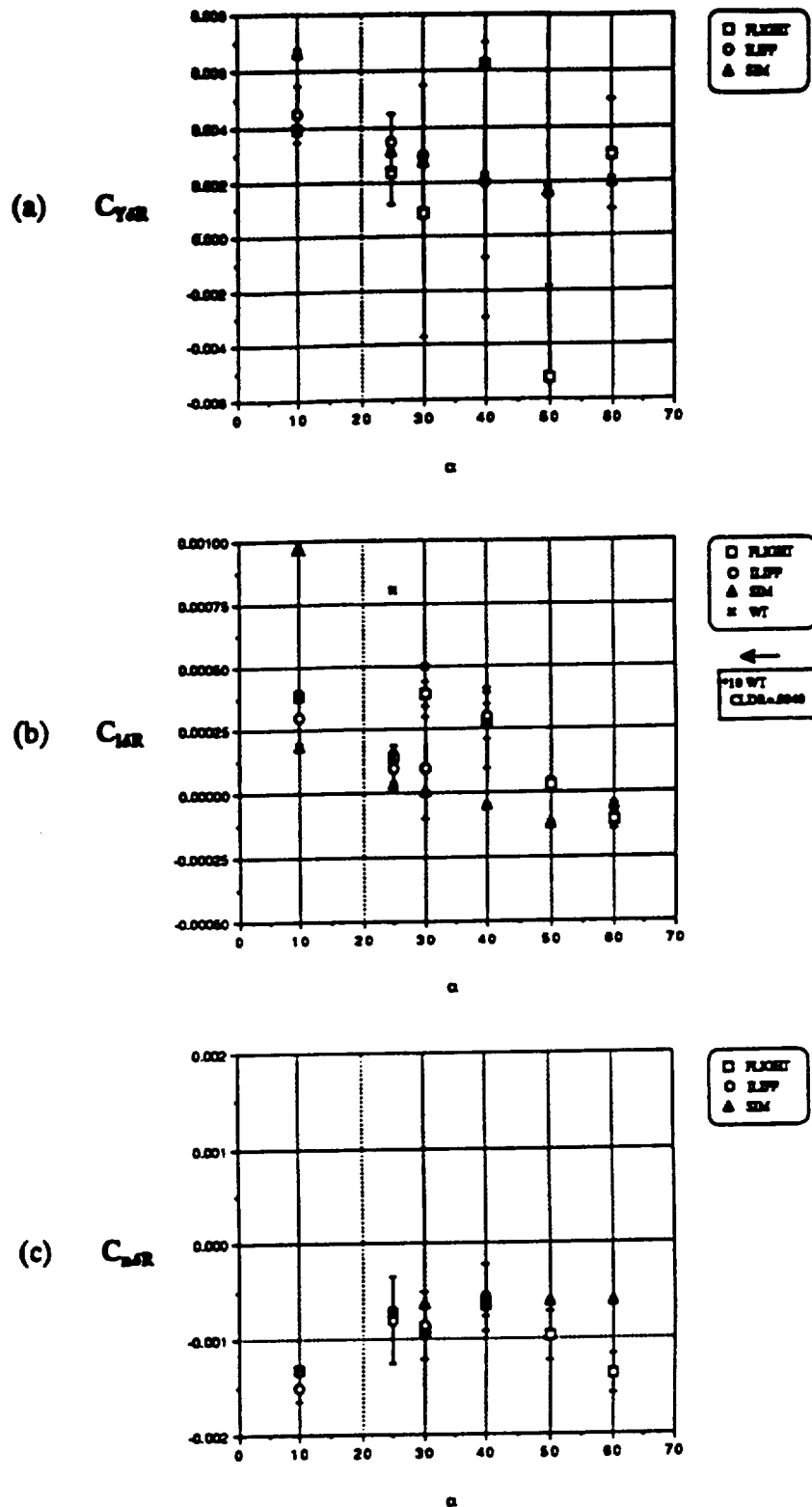
Figure 8.12: Rudder Derivatives (Lateral-Directional) (a) Lateral Force (b) Rolling Moment (c) Yawing Moment
