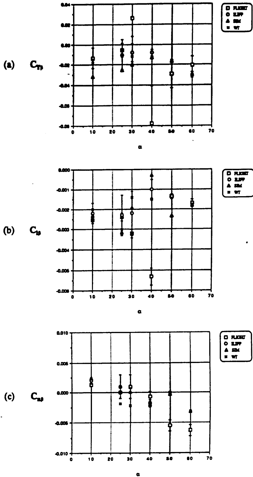
Figure 8.8: Sideslip Derivatives (Lateral-Directional) (a) Lateral Force (b) Rolling Moment (c) Yawing Moment
