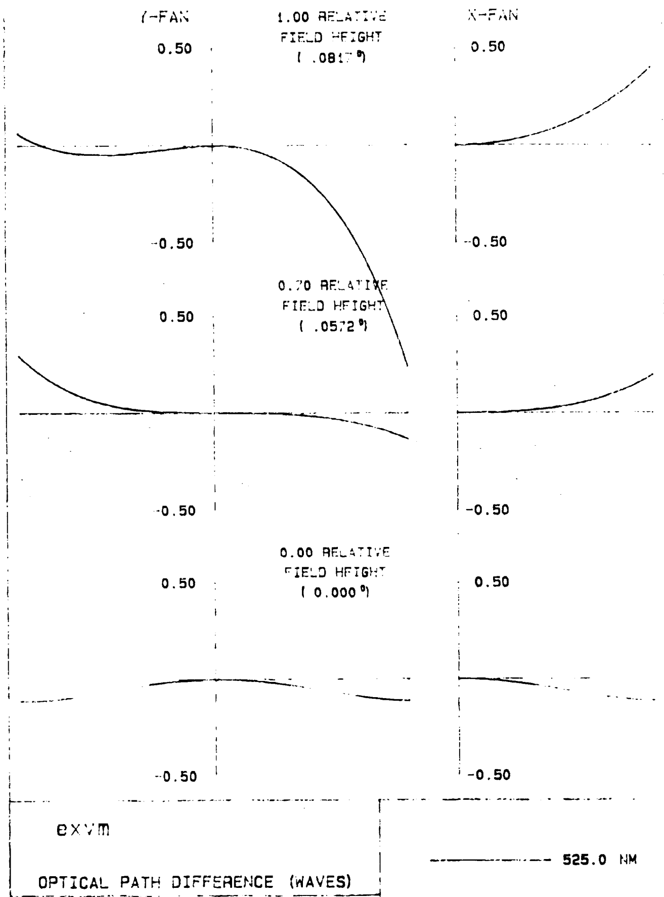
Figure 8: Wavefront aberrations of the EXVM in the final image plane.
