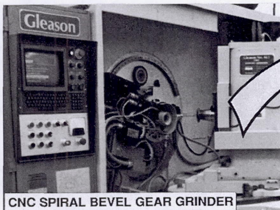
Figure 4.—Spiral bevel gear grinding.
