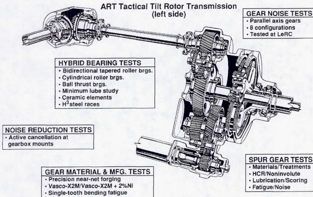
Figure 9.—Boeing Helicopter ART program component test plan.
