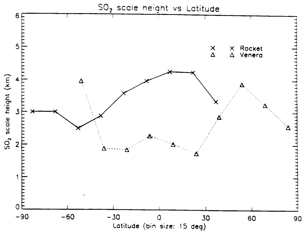
Figure 7: \text{SO}_2 mixing ratios and scale heights derived from Venera-15 and the sounding rocket observations are plotted against latitude. The results are binned in 15^\circ bins to reduce the scatter in the data.
