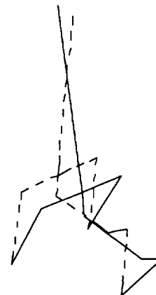
(f) Test-stand 2nd longitudinal mode at 7.23 Hz.
