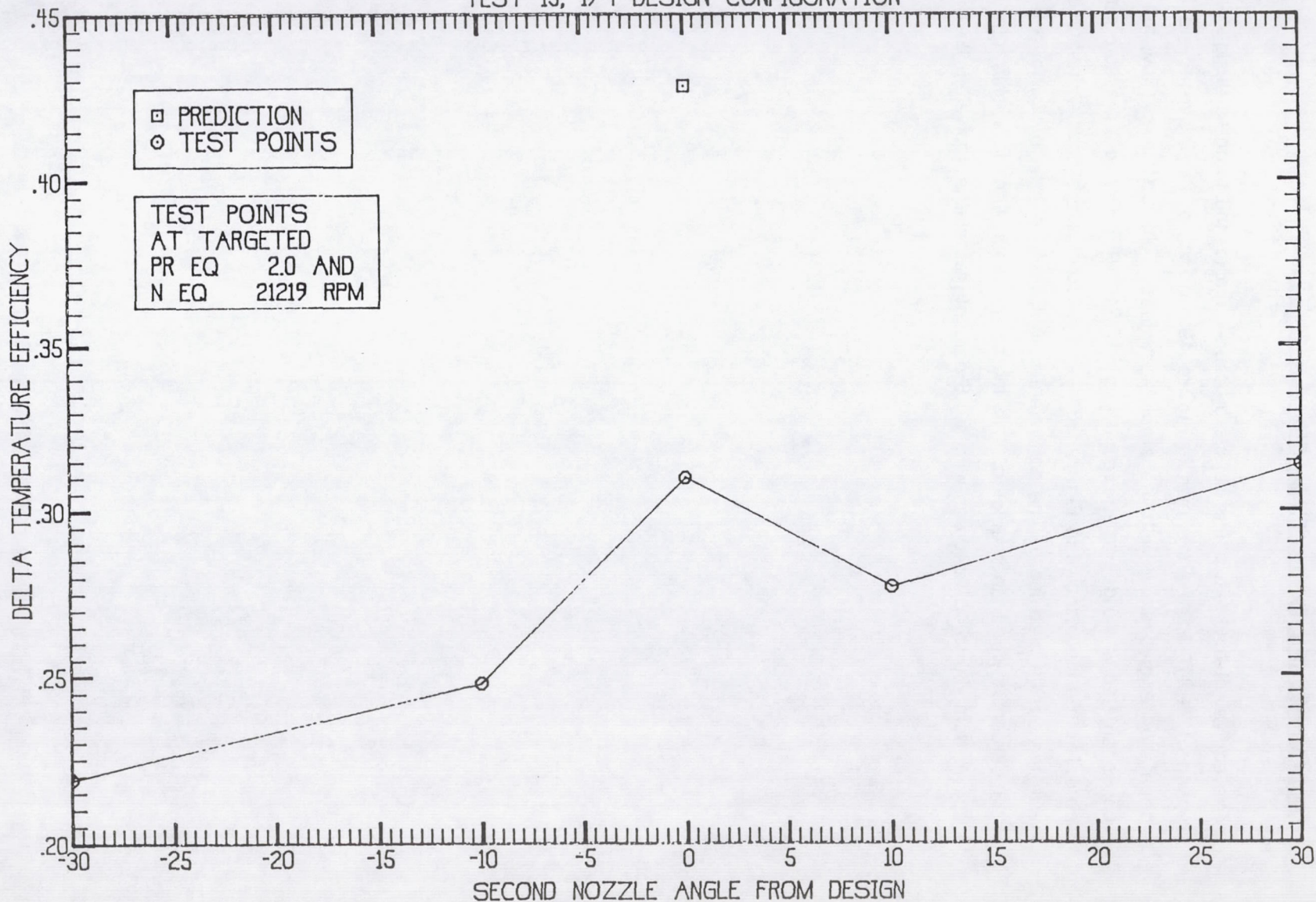
Figure 48 2 STAGE PARTIAL ADMISSION TURBINE TEST 13, 1/4 DESIGN CONFIGURATION
