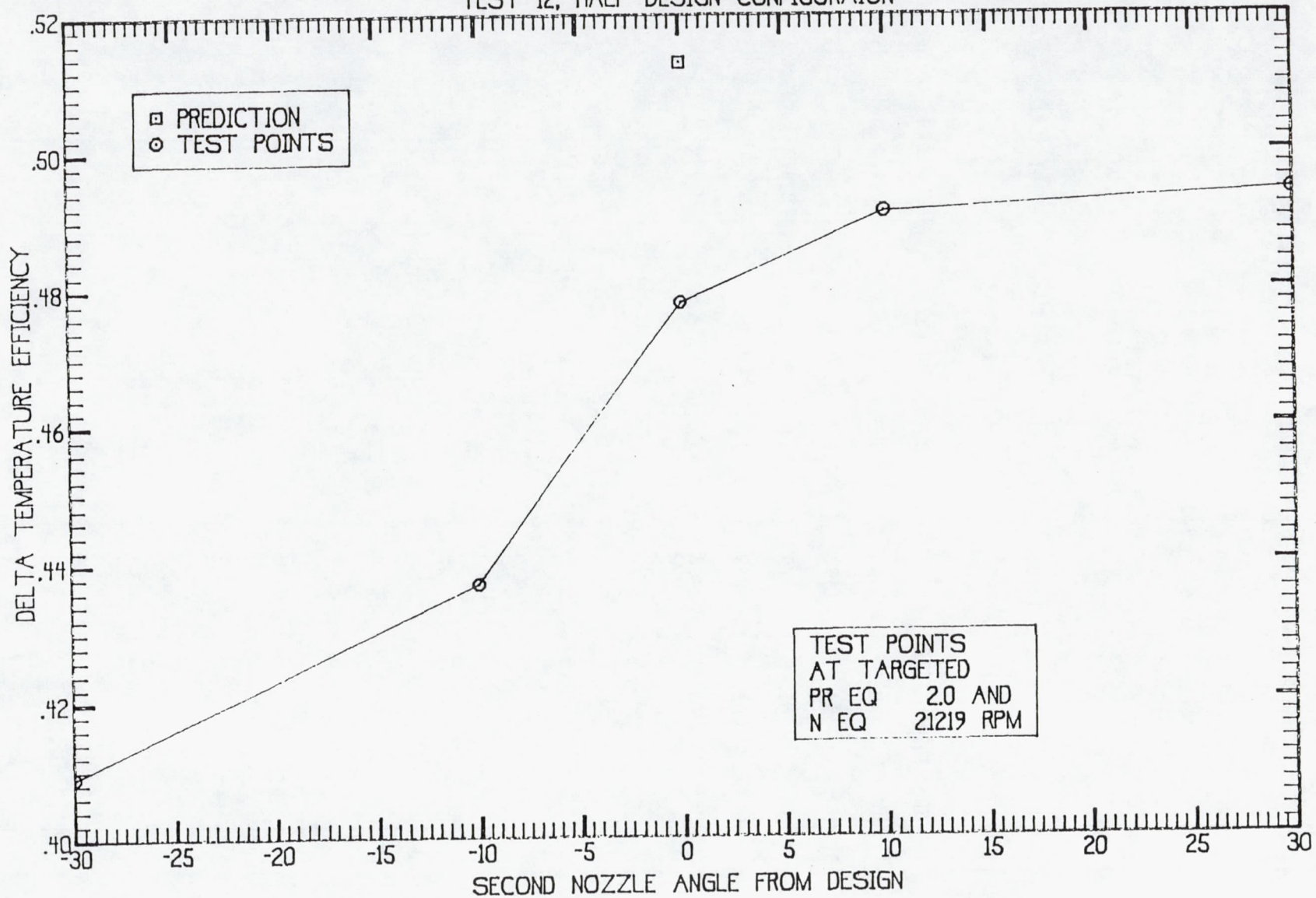
Figure 41 2 STAGE PARTIAL ADMISSION TURBINE TEST 12, HALF DESIGN CONFIGURATION
