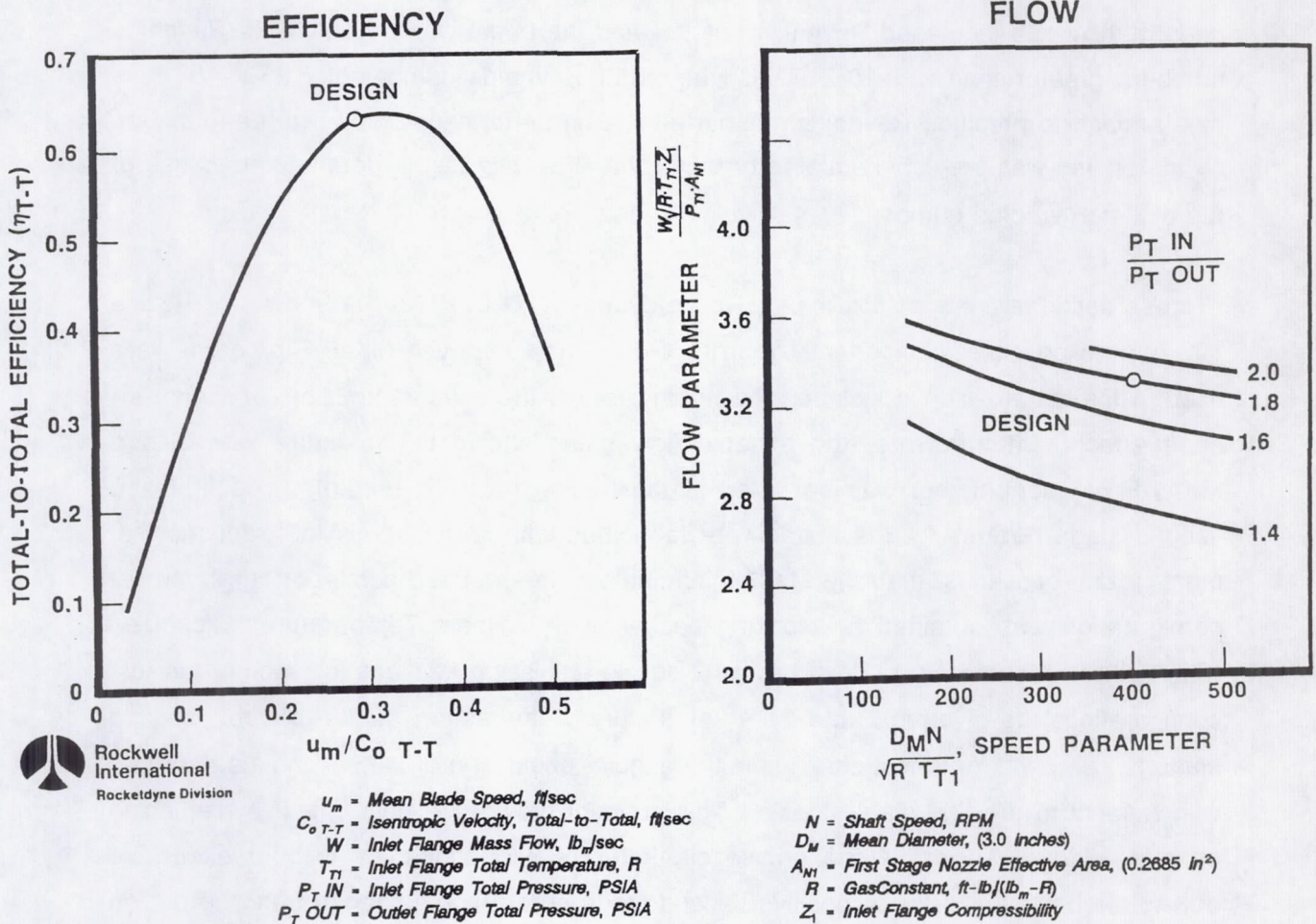
Figure 9 PERFORMANCE CHARACTERISTICS MARK 49-F TURBINE
