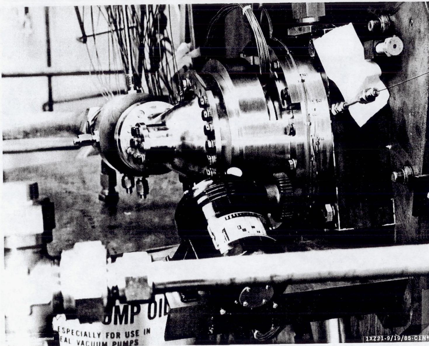
Figure 13 Second Stage Nozzle Angular Orientation Motor Drive Setup
