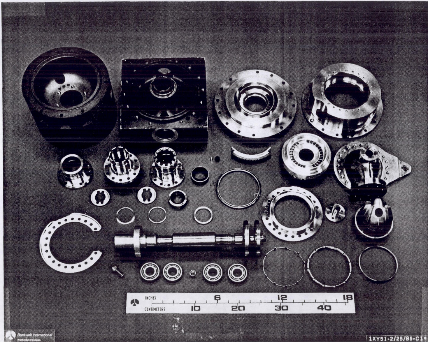
Figure 12 Tester Components
