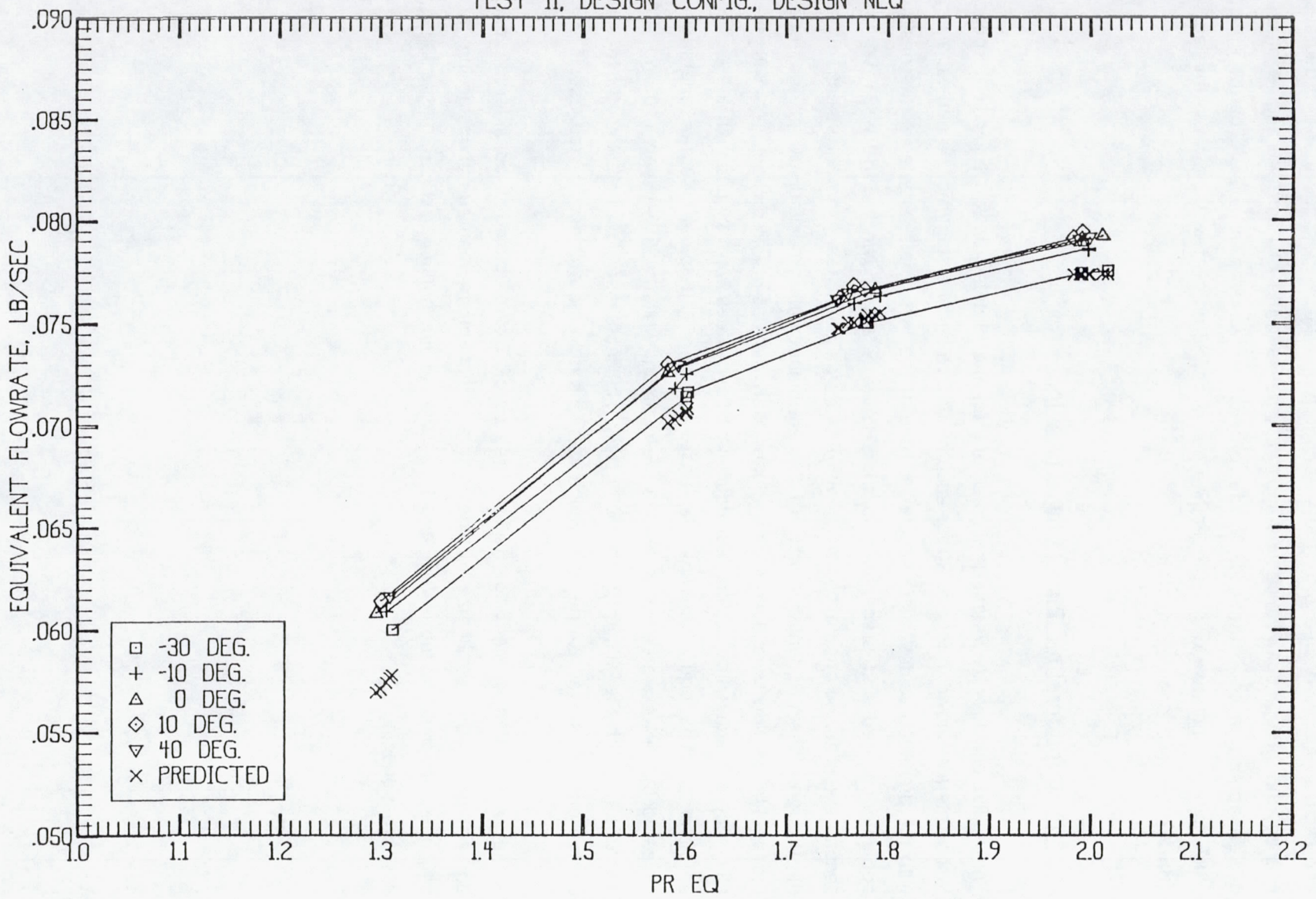
Figure 30 2 STAGE PARTIAL ADMISSION TURBINE TEST 11, DESIGN CONFIG., DESIGN NEQ
