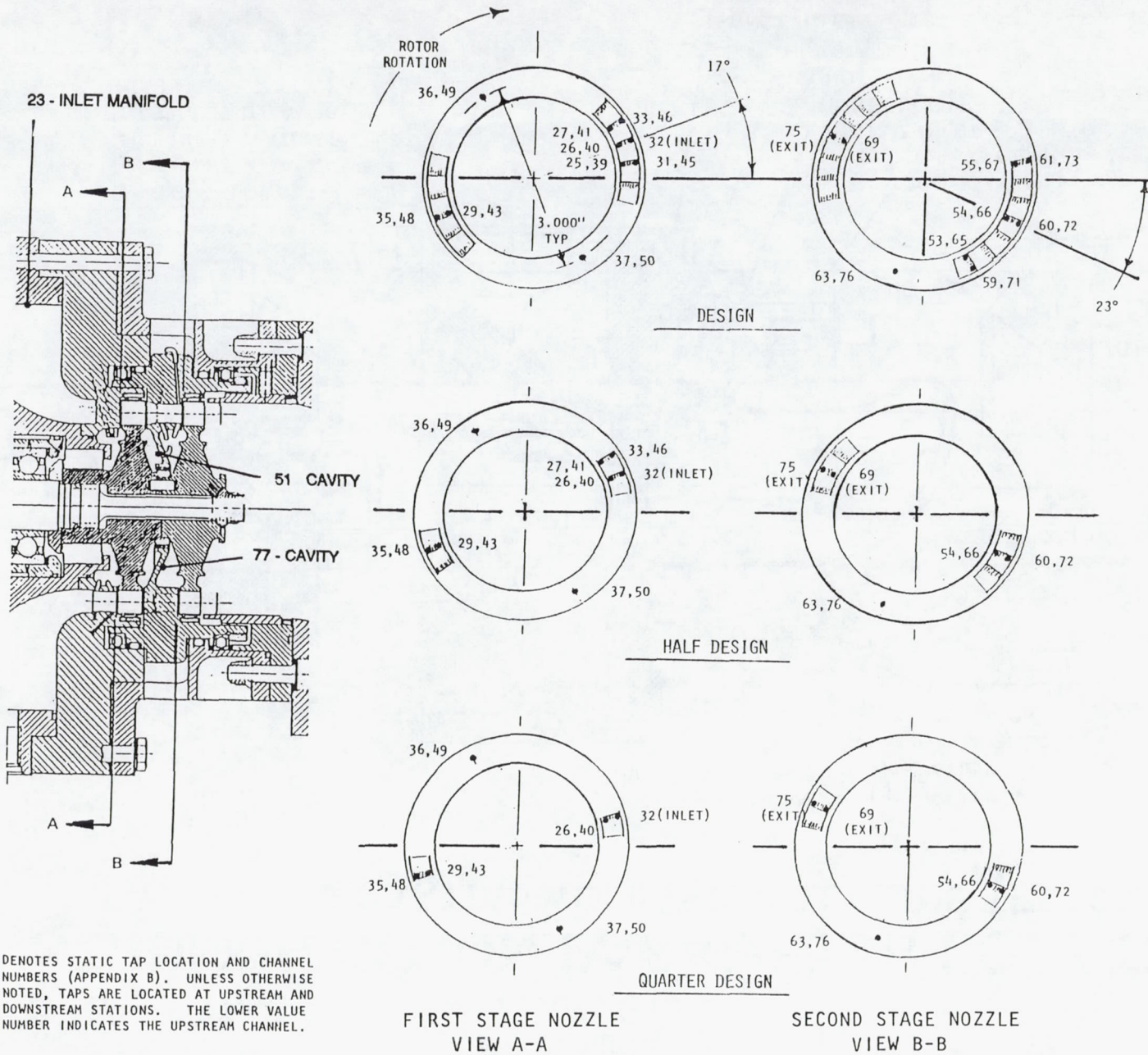
FIGURE 22 Static Pressure Tap Locations
