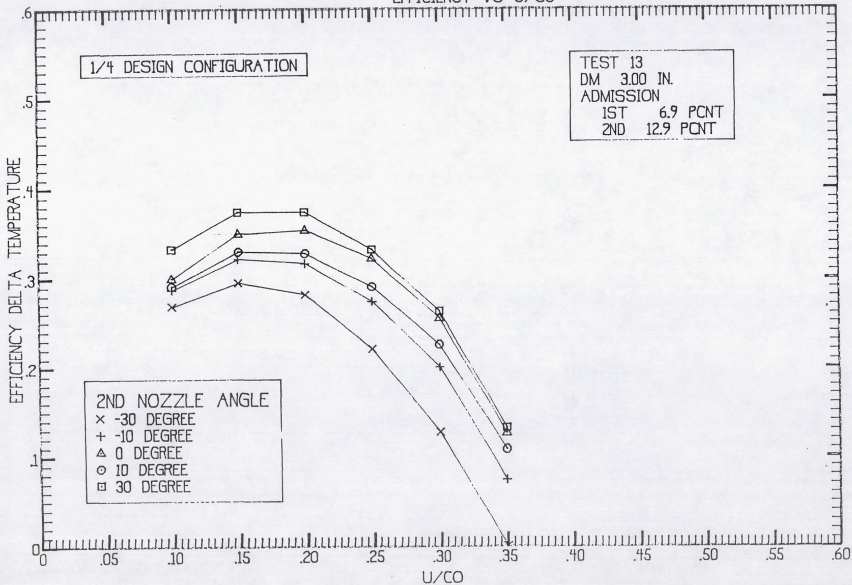
Figure 47 2 STAGE PARTIAL ADMISSION TURBINE EFFICIENCY VS U/CO
