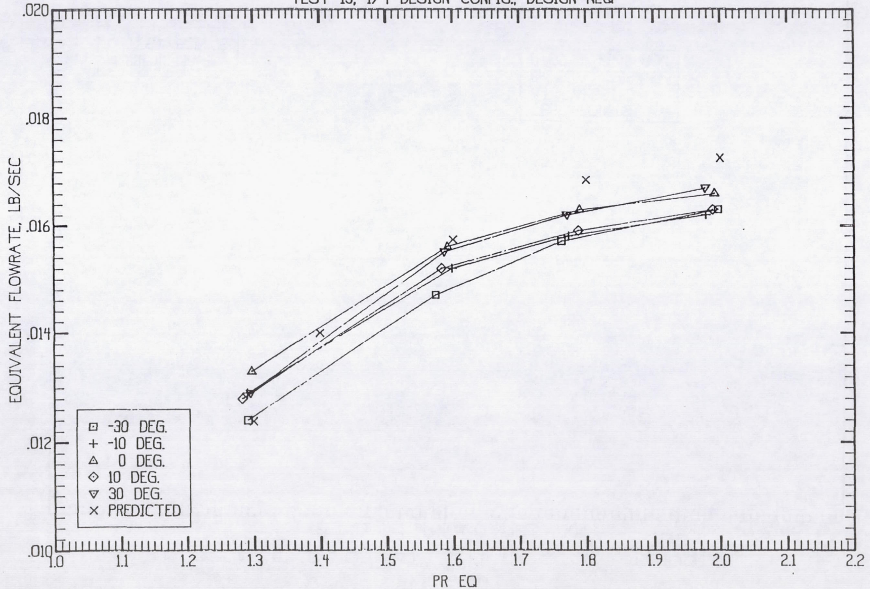
Figure 49 2 STAGE PARTIAL ADMISSION TURBINE TEST 13, 1/4 DESIGN CONFIG., DESIGN NEQ
