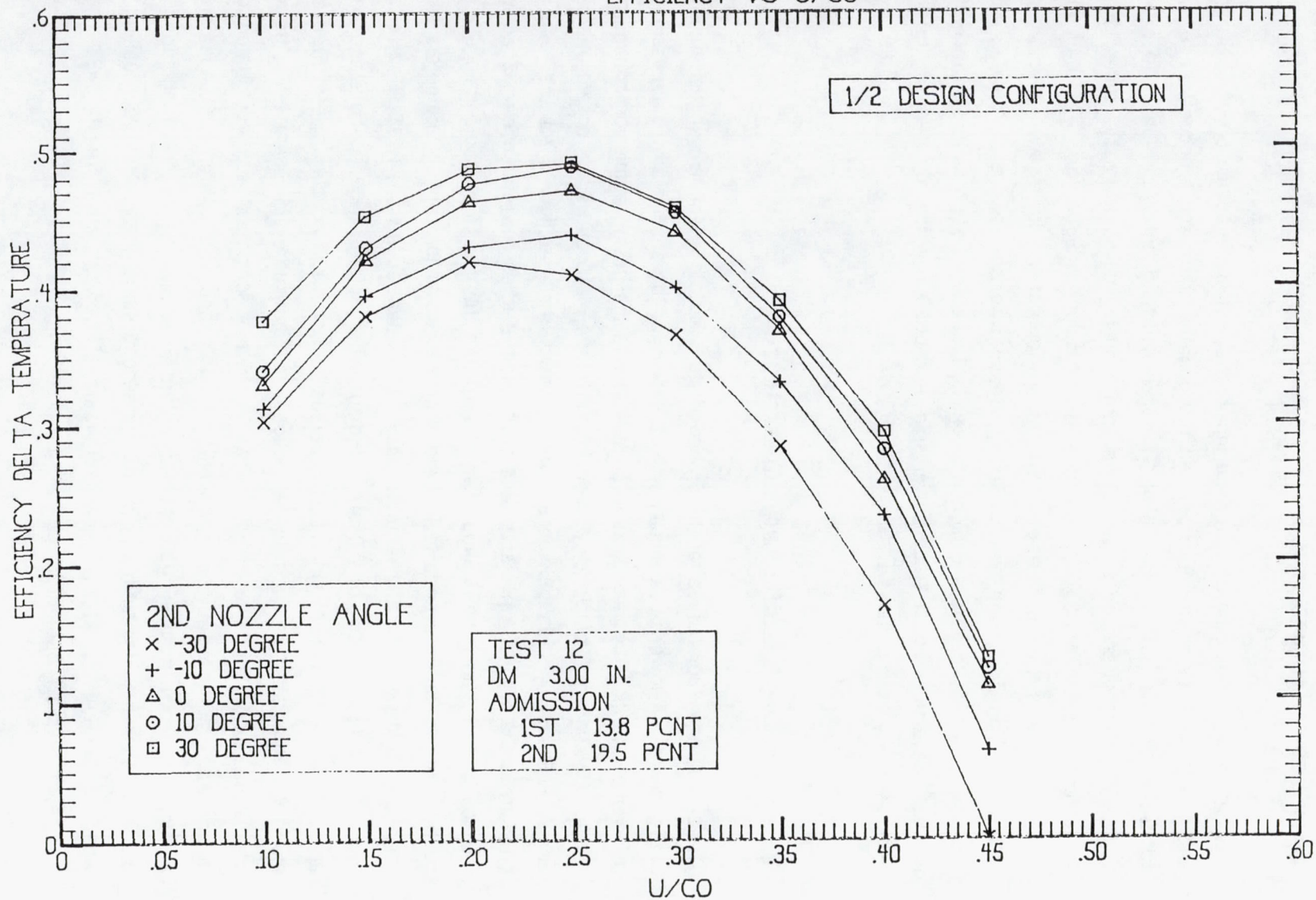
Figure 40 2 STAGE PARTIAL ADMISSION TURBINE EFFICIENCY VS U/CO
